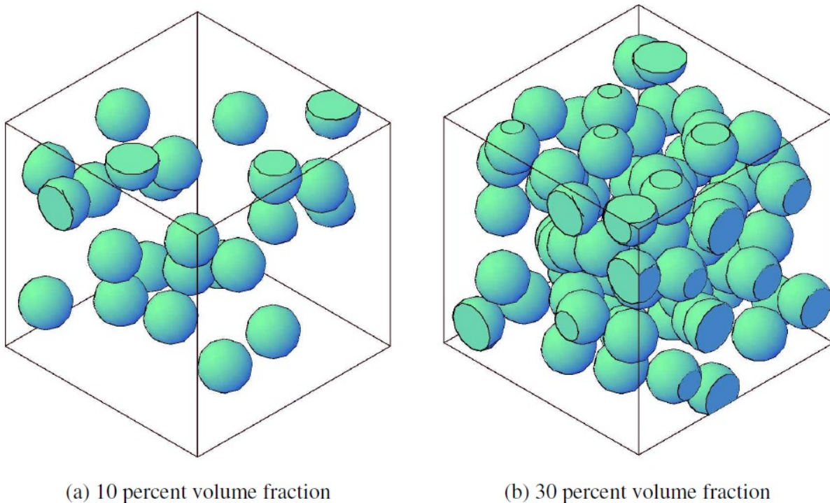
Figure 12 3D composite models with solid spherical particles
