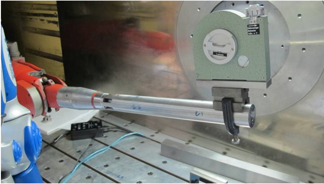
Figure 9: 120 mm clinometer measuring the arbor pitch angle
