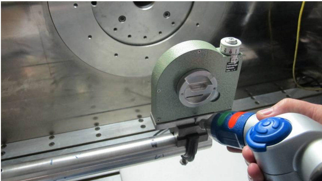
Figure 7: CMM measuring vertical position relative to centreline reference
