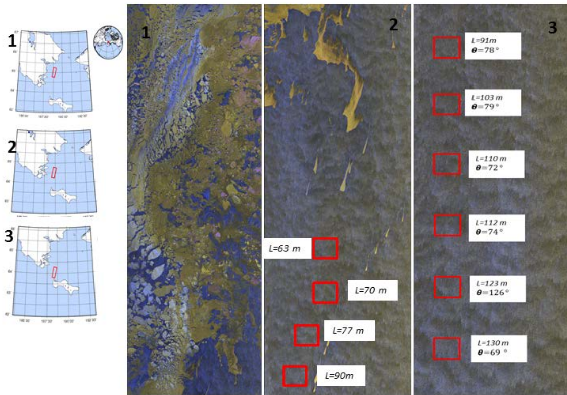
Figure 1: An example of the wave field in off-ice wind conditions in the Bering Sea (Dec 7, 2012), showing the increase in wave length L with increasing fetch
