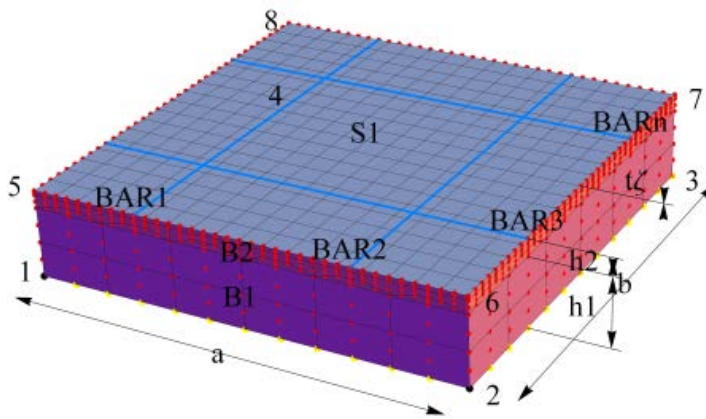
Figure 6. Solid representation of a 3-layer structure of dimensions a \times b \times (h_1 + h_2 + t) reinforced by 4 bar elements (BAR1, BAR2, BAR3 and BAR4)
