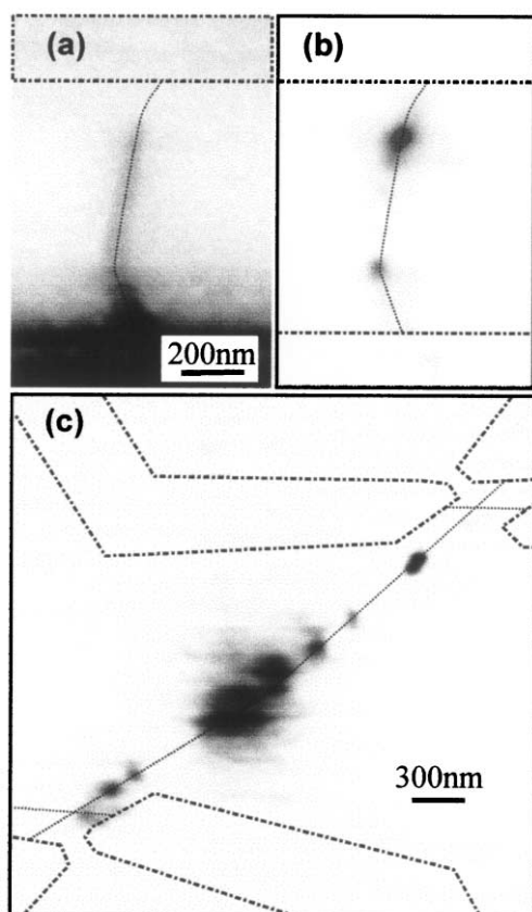
FIG. 4. (a) ac-EFM image of a 3 nm diameter semiconducting bundle of SWNTs (lines indicate the position of the bundle). The device resistance is approximately 60 M \Omega . An ac potential of 100 mV is applied to the lower electrode, while the tip is held at a dc bias of -2 V. (b) SGM image for V_{tip} = +1 V; black corresponds to immeasurably large resistance. (c) SGM image of a longer semiconducting SWNT bundle incorporated in a nanotube circuit (lines indicate the position of the bundle and the electrodes). Current is passed through the circuit from the upper left electrode to the lower right electrode.
