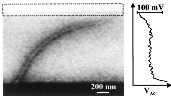
FIG. 3. An ac-EFM image of the same bundle of SWNTs shown in Fig. 1 before breaking. The bundle is metallic, with a total circuit resistance of 40 \text{ k}\Omega . An ac potential of 100 mV is applied to the lower electrode. The ac-EFM signal is flat along the length of the SWNT bundle. A trace of the potential as a function of a vertical position in the image is also shown.
