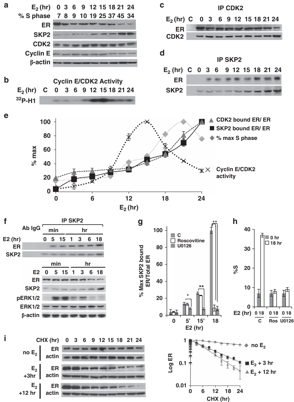
Figure 4. Quantitation of cyclin E-CDK2 activity, CDK2-bound and SKP2-bound ER \alpha and ER \alpha t_{1/2} during G1-to-S-phase progression. (a–e) E2-deprived MCF-7 were treated with 10^{-8} M E2 and recovered at intervals shown. (a) Flow cytometry showed cell cycle re-entry (% S phase), and western blots for ER \alpha , cyclin E, SKP2 and CDK2 are shown. \beta -Actin serves as loading control. (b) For cyclin E-CDK2 kinase activity, cyclin E was precipitated and reacted with histone H1 and radioactivity in substrate ( ^{32} P-H1) shown by autoradiography. Activity was quantitated by phospho-imager and graphed as mean % max activity \pm s.e.m. from >3 assays in (e) below. (c, d) CDK2-bound ER \alpha (c) and SKP2-bound ER \alpha (d) assayed at intervals after E2 addition. (e) Quantitation of data from a–c above. The experiments were repeated at least three times. Data were normalized to highest read, and graphed as mean % max \pm s.e.m. from >3 assays. (f) E2-deprived MCF-7 were treated with E2 for intervals shown, lysed and assayed for SKP2-bound ER \alpha . Lanes 1 and 2 are antibody control and normal immunoglobulin G control for IP. Lower panel shows input on western blot. (g) SKP2-bound ER \alpha was assayed at intervals after E2 addition \pm pre-treatment with CDK2 inhibitor Roscovitine or MEK inhibitor U0126, and graphed as mean % max \pm s.e.m. from >3 assays (see also Supplementary Figure S2). Significance was determined using a two-tailed Student's t -test by comparing control with that from drug pre-treatment (* P<0.05 or ** P<0.01 ). (h) Flow cytometry (% S phase) showed cell cycle re-entry at 18 h in control but not in drug treated cells. (i) E2-deprived MCF-7 were treated with E2 for 3 or 12 h before adding CHX and harvested at various time points for ER \alpha western blot. \beta -Actin serves as loading control. After 3 h of E2, ER \alpha has a t_{1/2} of 6 h, whereas after 12 h of E2, ER \alpha has a t_{1/2} of 5 h.
