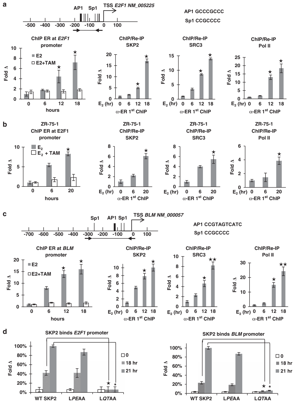
Figure 6. SKP2 directly regulates late ER \alpha -activated genes E2F-1 and BLM . MCF-7 or ZR-75-1 cells were harvested after 48-h E 2 deprivation at time = 0 h or after 10 nM E 2 for the times indicated. (a, b) ER \alpha ChIP was performed at the E2F-1 promoter at indicated times in MCF-7 (a) or ZR-75-1 (b) . ER \alpha ChIP/Re-IP used SKP2, SRC3 or polymerase II (Pol II) Abs for the re-precipitation. The fractions of protein bound to the promoter at different E 2 treatment intervals were compared with that of E 2 depleted cells and significant differences were determined using a two-tailed Student's t -test (* P < 0.05). (c) ER \alpha ChIP was performed at the BLM promoter. ER \alpha ChIP/Re-IP used antibodies to SKP2, SRC3 or Pol II. The fractions of protein bound to the promoter at different E 2 treatment intervals were compared with that of E 2 depleted cells and significant differences were determined using a two-tailed Student's t -test (* P < 0.05 and ** P < 0.01). (d) MCF-7 cells stably expressing Xpress-tagged WT SKP2, SKP2-L 114 PEAA 118 or SKP2-L 248 QTAA 252 were harvested after 48 h E 2 deprivation at time = 0 h or after 10 nM E 2 treatment for 18 or 21 h. ChIP experiments were performed at E2F-1 or BLM promoters using anti-Xpress antibody. Significance was determined using a two-tailed Student's t -test by compared the fraction of WT-SKP2 protein binding to gene promoter at 18, 21 h of E 2 with that of cells expressing SKP2 L 248 QTLL 252 (*, * P < 0.05).
