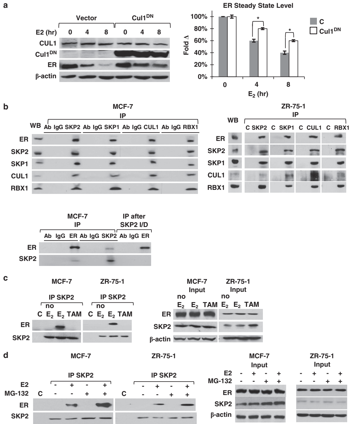
Figure 1. SCF SKP2 binds ER \alpha on estrogen stimulation. (a) MCF-7 cells were transfected with vector ( c ) or Cul1 DN , E2-deprived 48 h then treated with 10^{-8} M E2 for 4 or 8 h. Western blots show ER \alpha and CUL1, with \beta -actin loading control. Data from three independent experiments performed in triplicate were plotted as percentage of remaining ER \alpha level ( \pm s.e.m.) relative to ER \alpha level at the time of E2 depletion. Significance was determined using a two-tailed Student's t -test (* or * P < 0.05). (b) Immunoprecipitations (IP) of indicated SCF SKP2 components were performed using 1 mg total cell lysate and associated proteins detected by blotting in MCF-7 (left) and ZR-75-1 cells (right). Antibody without lysate served as control (Ab or C). Nonspecific polyclonal antibody failed to precipitate these proteins (immunoglobulin G). To estimate the amount of ER \alpha associated with SKP2, cell lysates were immunoprecipitated with either anti-ER \alpha antibody, with anti-SKP2 antibody or with anti-SKP2-conjugated beads after three serial immunodepletions with anti-SKP2-conjugated beads (see lower panel). (c) E2-deprived MCF-7 and ZR-75-1 cells were treated with vehicle (no E2), 10^{-8} M E2, or 10^{-5} M 4-hydroxytamoxifen (TAM) for 1 h. Lysates were assayed for SKP2-bound ER \alpha (left, lane 1 is IP control as above). Right panel shows input on western blot. (d) E2-deprived MCF-7 and ZR-75-1 were treated \pm E2 for 1 h, \pm MG-132 addition immediately before E2, lysed and assayed for SKP2-bound ER \alpha . Lane 1 is control as above. Right panel shows input on western blot.
