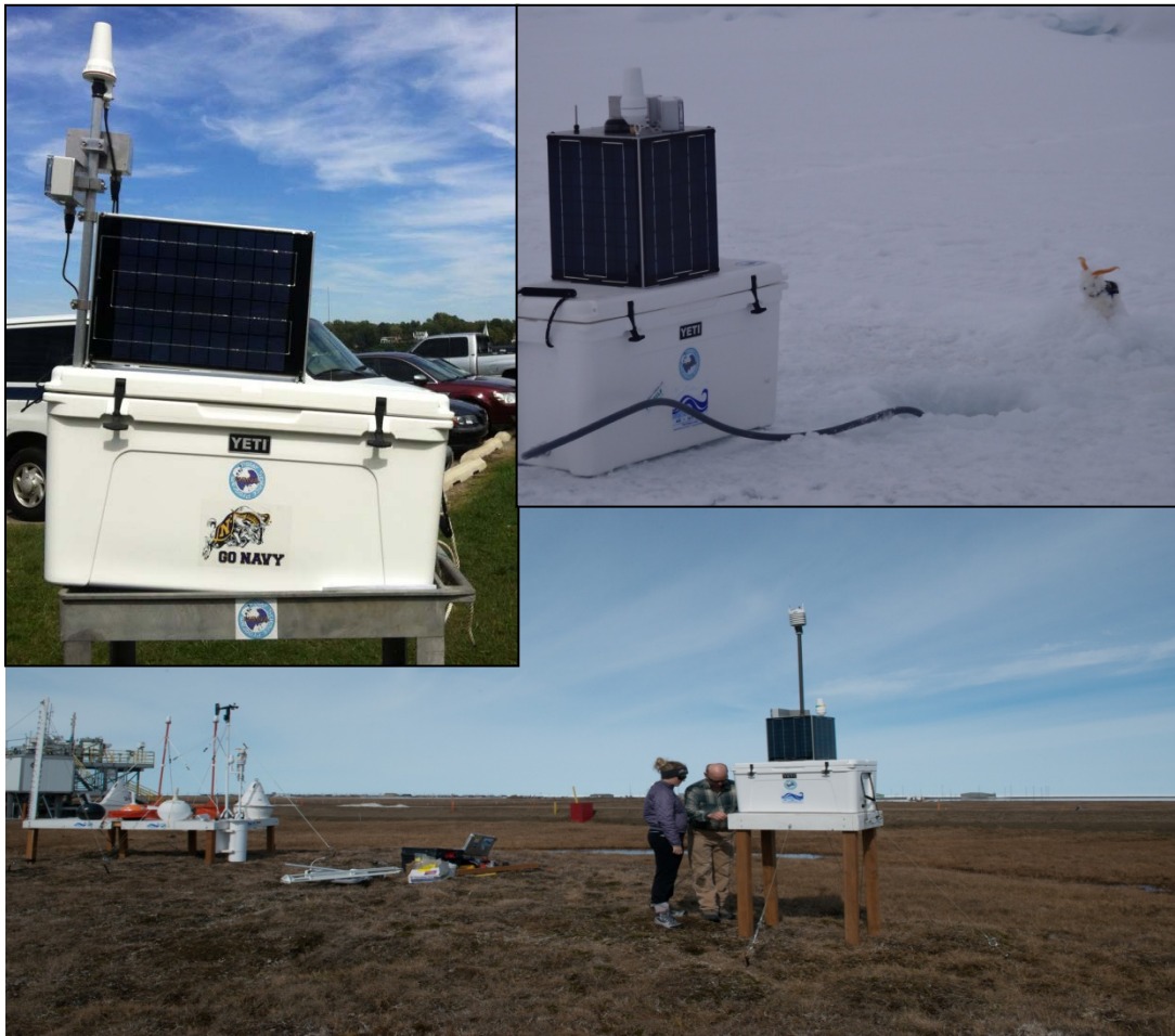
Figure1: (top left) IK1 undergoing testing at USNA; (top right) IK2A with hydrophone through the sea ice offshore Barrow, AK.; (bottom) IK3T at AOX site in Barrow, AK. The AOX site is monitoring temperature biases between all buoy systems currently operated by the International Arctic Buoy Program (IABP). Mishipman Julia Zook works with University of Washington Engineer Jim Johnson on the IK3T during her summer internship to Barrow, AK.
