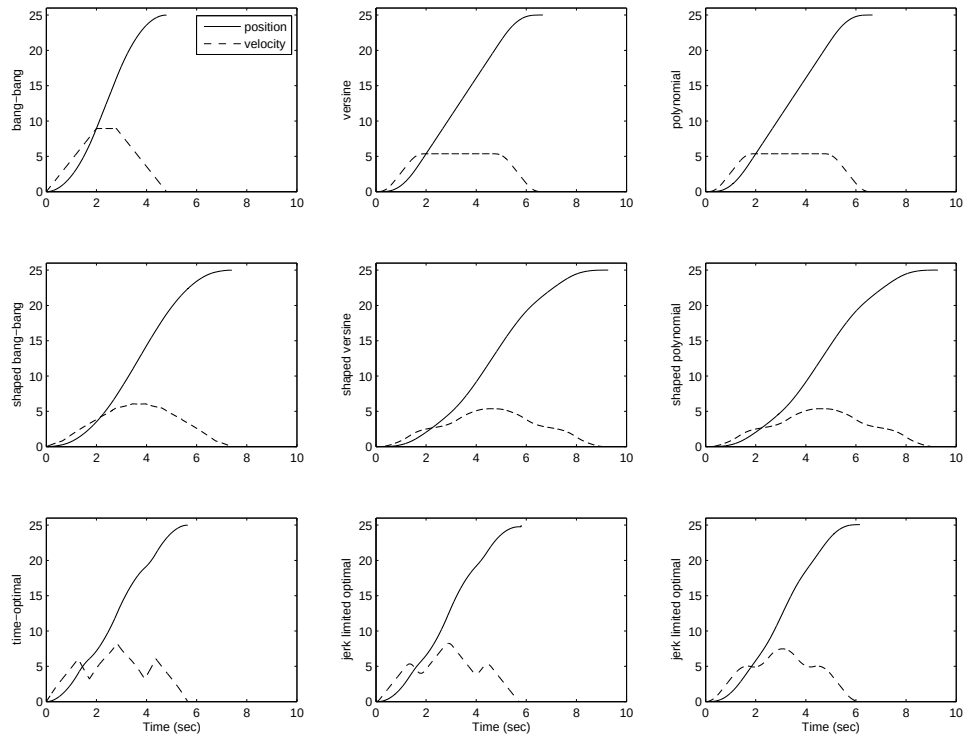
Figure 18. Reference Trajectory
