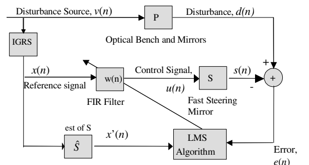
Fig. 4 Block diagram of the FXLMS control system. The IGRS is a sensor/signal generator that synthesizes a reference signal for the algorithm.
