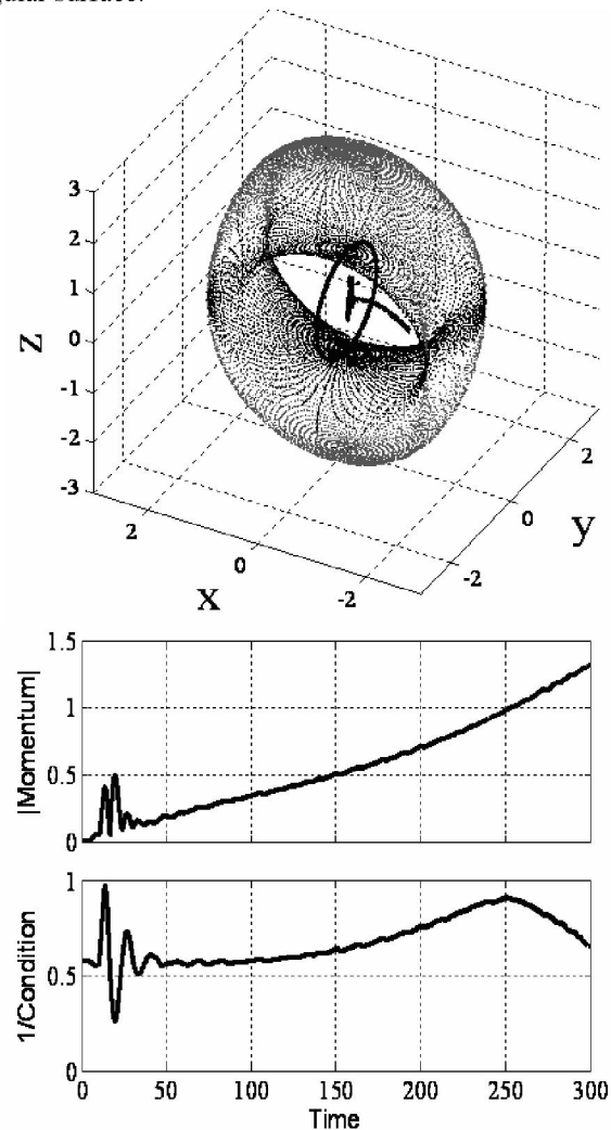
Fig. 11. Experimental results: +5^\circ yaw in 4 seconds, -5^\circ yaw in 4 seconds, then regulate at \{x,y,z\} = \{0,0,0\} countering cg-offset disturbance torque of unbalanced ground test satellite simulator. Momentum trajectory placed in context of theoretical singular momentum hypersurface of \beta_1=90^\circ configuration. Magnitude of normalized momentum and inverse of condition number of [A] matrix (would approach zero if array became singular).
