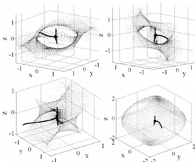
Fig. 12. Experiment from Fig. 11 performed in \beta_i=90^\circ configuration placed in context of “optimal spherical” \beta_i=54.73^\circ for the purpose of comparison (plots rotated for clarity). Note continuous flirting with singular surfaces and impact with surface occurs less than \frac{1}{4} way through trajectory. This trajectory would not have continued as depicted had the skew angles been \beta_i=54.73^\circ . Instead the array would have gone singular and attitude control would have been lost.
