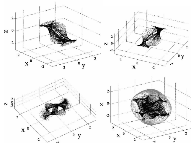
Fig. 6. Singular surfaces for 3/4 CMG skewed array at “optimal spherical” momentum skew angle \beta=54.73^\circ . Top: 1H & 2H surfaces; Bottom left: 1H & 2H surface; Bottom right: 1H & 2H surfaces inside 0H & 3H surfaces.
