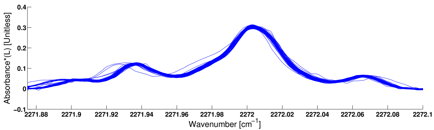
Figure 6.12: In these plots the natural log of \frac{I}{I_0} is taken for both CO (top) and CO 2 (bottom). Concentration for each molecule is found by dividing the area under the region of interest by the pressure, path length, and temperature dependent line strength. This data is at an equivalence ratio of 1.5, a height above the burner of 5mm, and a repetition rate of 10 kHz.
