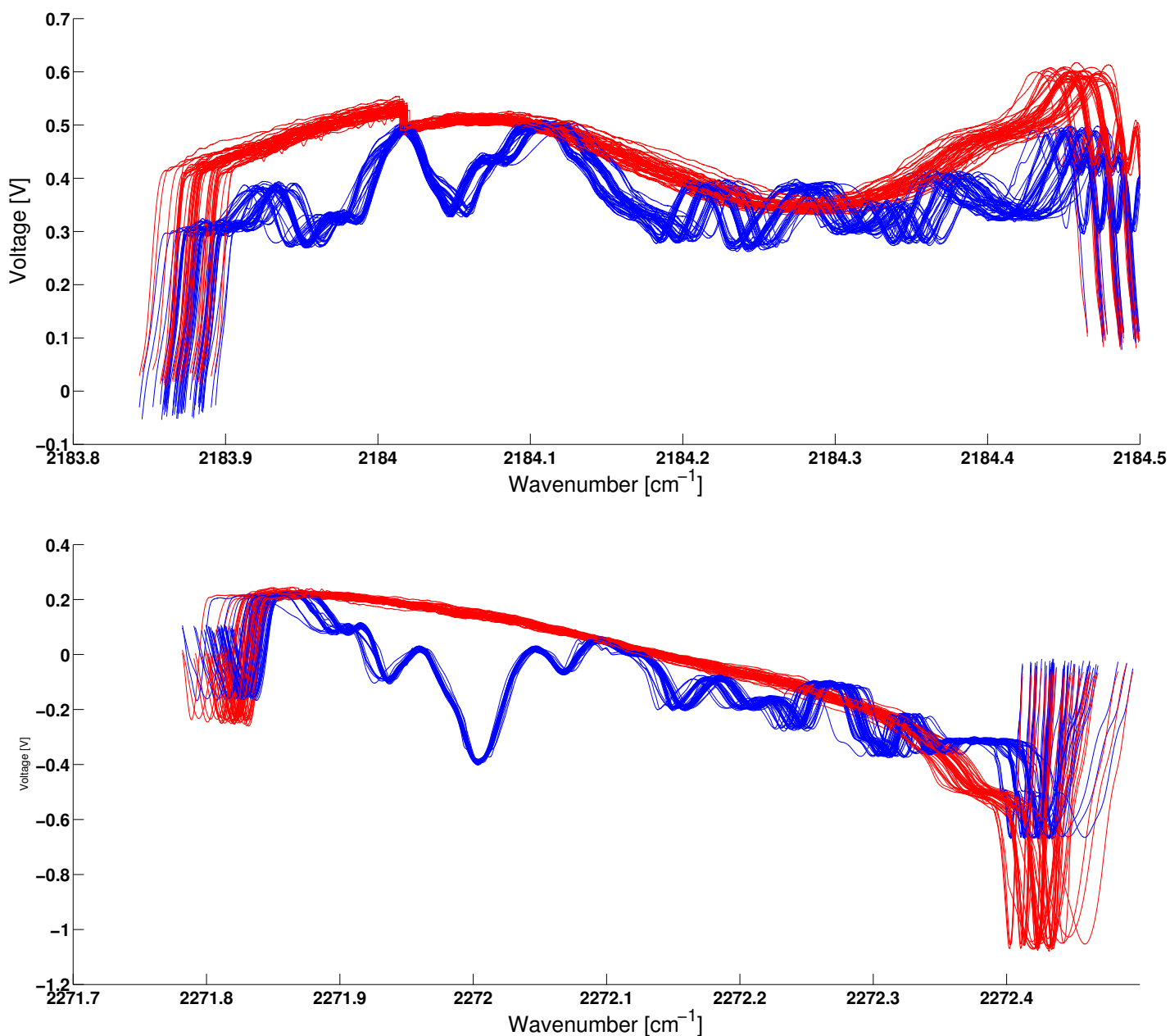
Figure 6.6: Plots showing a properly adjusted " I_0 " (red) for both CO (top) and CO 2 (bottom). The red line is the laser intensity with no absorption; however, unlike in the raw data it has been adjusted to line up with zero absorption. That is, the region with no absorption is adjusted vertically to line up with the relative voltage maximums (which correspond to zero absorption) near the peaks of interest. This data is at an equivalence ratio of 1.0, a height above the burner of 5mm, and a repetition rate of 10 kHz.
