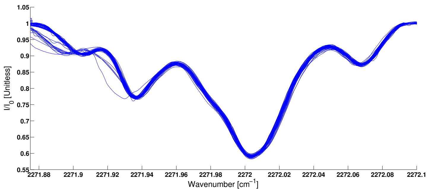
Figure 6.8: Data for CO (top) and CO 2 (bottom) in which the intensity is normalized according to an intensity where no absorption occurs according to Beer's Law. Furthermore, the plots now focus on the regions of interest. For an equivalence ratio of 0.7, height above the burner of 5mm, and repetition rate of 10 kHz, it can be seen that the CO peak is not discernible. It is therefore not detectable and there is more experimental error associated with the 50 data sets in this sample.
