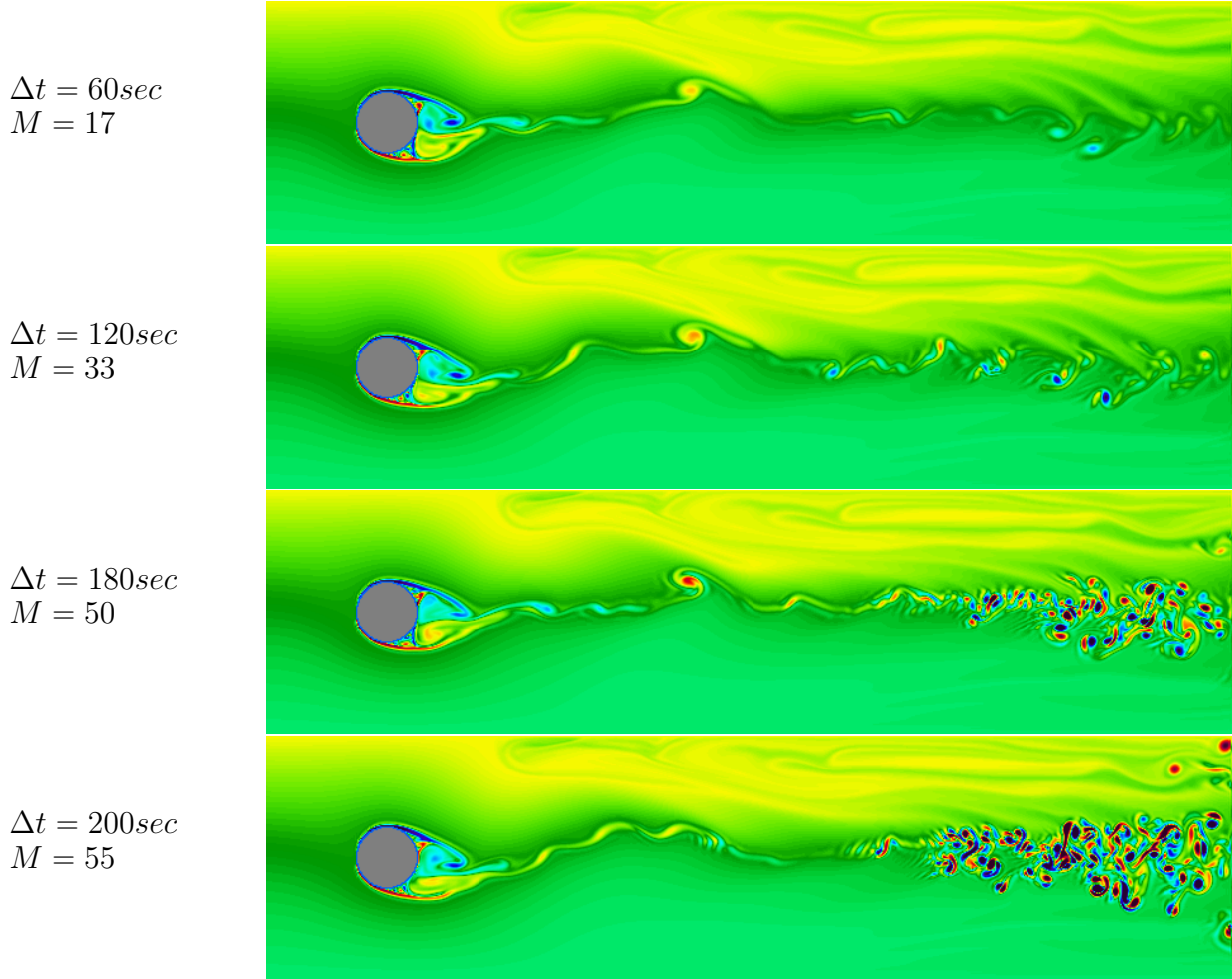
Figure 5: An example of weak numerical instability caused by inaccurate mode splitting. All the conditions are the same as in Fig. 4, the second panel from the bottom, \Delta h = 275\text{m} , except that in this simulation vertically averaged velocity components participating in computation of r.h.s. terms for 3D momentum equations are time centered at n th step (not extrapolated to n + 1/2 ), and there is also no recomputing of advective terms at every time step within the barotropic mode. \Delta t indicated on the left of each panel is the time step for 3D mode, and M is the mode splitting ratio (the barotropic time step \Delta t/M is approximately the same for each panel). Notice a non-physical instability of the wake, which is strongly dependent on the size of the time step. Consistent mode splitting (either extrapolated vertical averages or recomputed barotropic advective terms) do not exhibit such sensitivity.
