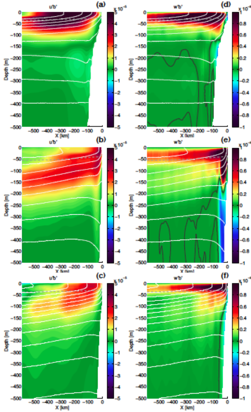
Figure 1: Annual and along-shore averages of across-shore (left) and vertical (right) eddy buoyancy flux [ \text{m}^2 \text{s}^{-3} ] for the Peru (top), Chile (middle), and California (bottom) current systems. White contours are the mean buoyancy field, and the gray dashed line is the boundary-layer depth diagnosed by the K-Profile Parameterization. Black contours are vertical flux w'b' = 0 . The eddy flux patterns are generally shoreward in u'b' and upward in w'b' , acting to balance the air-sea heating and mean upwelling circulations. While there is general qualitative similarity across the regions, there are noticeable regional differences in stratification and fluxes. (Colas et al., 2013a)
