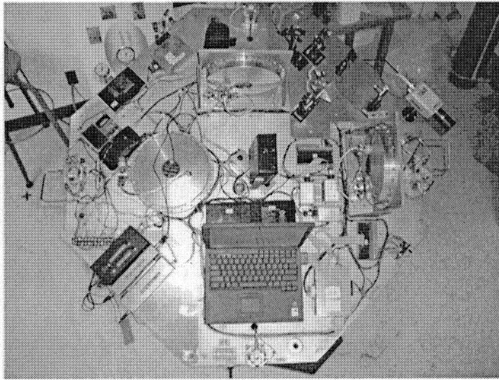
Figure 8. TASS Top View
