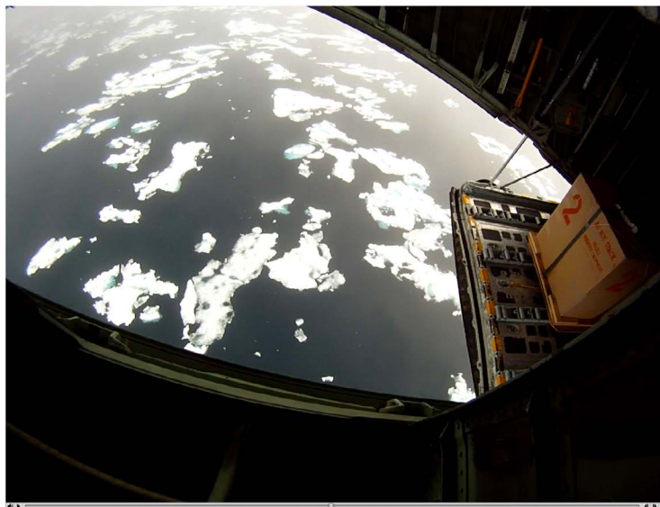
Figure 2. View out the open ramp from the proposed location of the VarioCam InfraRed camera. The large box is an UpTempO buoy that is about to be deployed. The actual field of view of the VarioCam is much smaller and will mostly include just the open area at an oblique angle.
