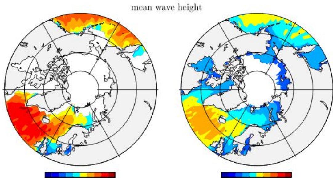
Figure 1. Mean wave height in the Arctic Seas, over 2002-2012. (left) March, (right) September
