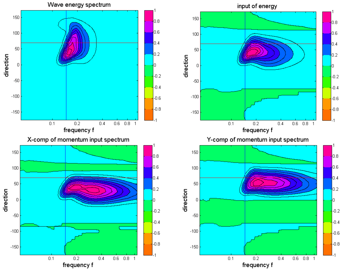
Figure 4 demonstrates testing the WBL module for WAVEWATCH-III. Realistic hindcast spectra are used (top left), for the U_{10} wind speed of 10.6m/s. The wind energy-input spectrum (right) is shown in top right, and the two components of the wind momentum-input spectra at the bottom. All the input spectra have positive and negative lobes. All spectra are normalised for the comparison.
