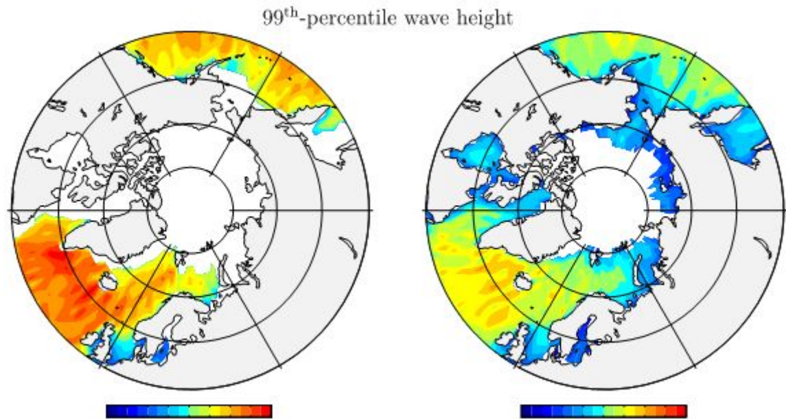
Figure 2. Extreme wave heights (top 1%) in the Arctic, 2002-2012. (left) March, (right) September
