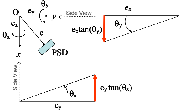
Figure 9. Contribution to the f readings due to small tip and tilt top plate motion
