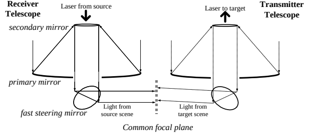
a) High level scheme of the optical subsystem
