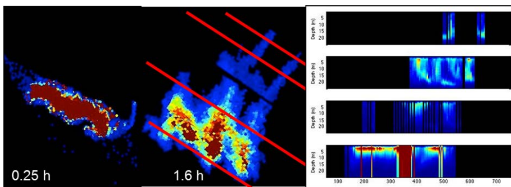
Figure 5 Moderate Strain region, surface injection, June 16, 2011, selected Fluorescein composite plan view of peak lidar dye return intensity 0.25 hours and 1.6 hours after initial dye injection (left. Red lines indicate location vertical profiles. The lidar vertical profiles (right) plotted North to South (top to bottom, respectively) indicate rapid mixing down and subduction of the dye. Return intensity is color coded such that details outside of the core of the dye patch can be readily seen
