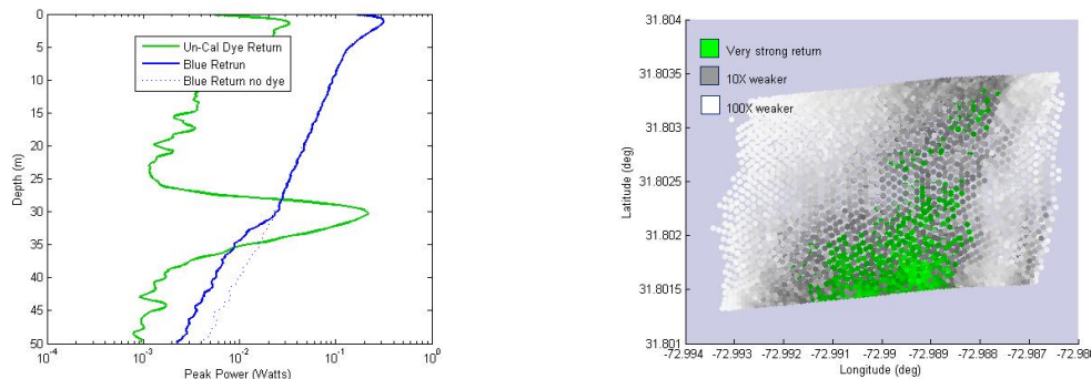
Figure 2 To the left, an example of the dye return signal (green) and lidar backscattered return signal (blue), sampling water with (solid) and without dye (dotted). To the right, geo-registered lidar dye returns from a single flight pass, the dye return strength varies from the central core to the edges of the streak by several orders of magnitude, indicating similar dye concentration variations.
