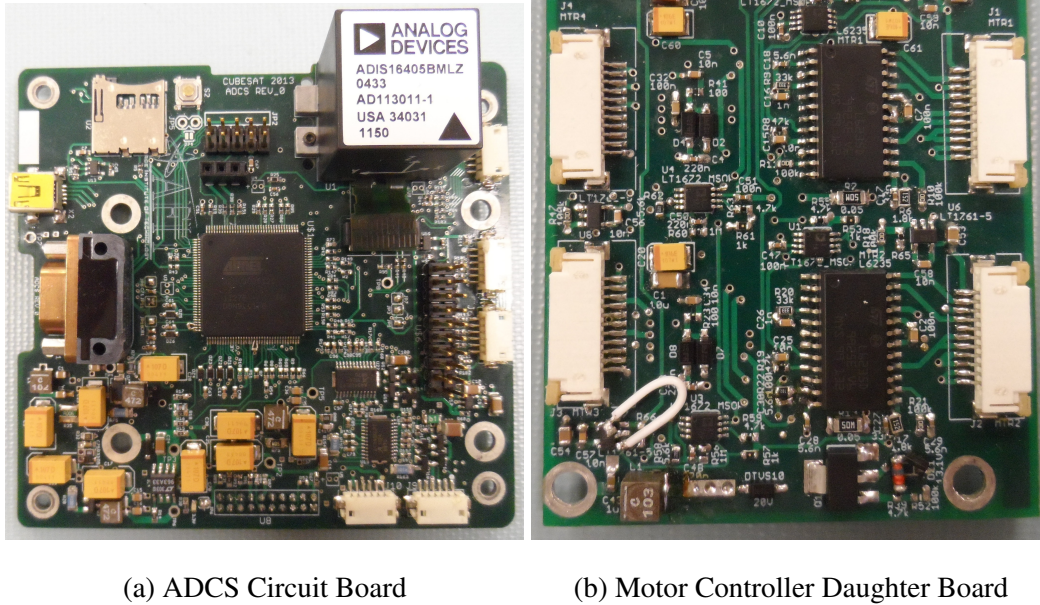
Figure 3.16: ADCS Circuit Board Configurations
