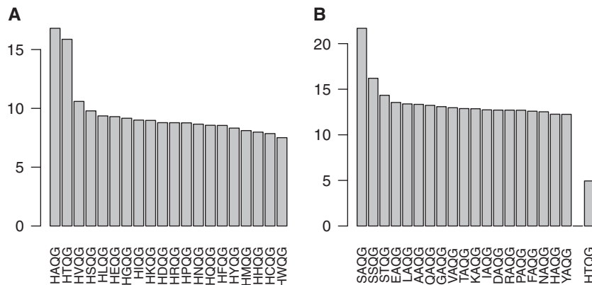
FIG 8 Fitness landscapes of an HA protein 4-aa segment inferred from MSA. (A) H5 landscape derived from H5N1 sequences. (B) H3 landscape from H3 sequences. The height of the bars represents the fitness values in units of r_s = 1.0 \text{ day}^{-1} . The abscissa shows the list of genotypes sorted with decreasing order in fitness. In panel B, the rightmost bar shows the H5 WT, which is 251st in rank.
