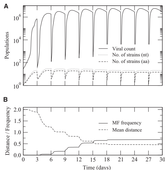
FIG 3 Time dependence of population size and diversity (A) as well as mean distance to the MF sequence and the frequency of the MF (B). Parameter values were as follows: L_a = d = 2 aa, V_0 = 1 \times 10^4 , U_0 = 1 \times 10^6 , a = 1.0 \times 10^{-3} \text{ day}^{-1} , b = 1.0 \text{ day}^{-1} , r_0 = 20 \text{ day}^{-1} , \mu = 1.0 \times 10^{-5} , and \tau = 3 days.
