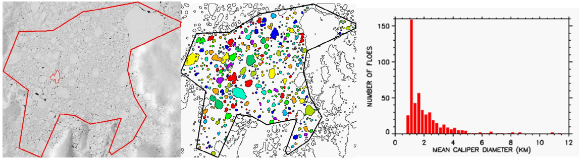
Figure 4. Left: MODIS image subset, band 3 (visible), from July 7, 2013, near 80°N 180°W, measuring 143 \times 125 km ( 571 \times 501 pixels). The heavy red outer curve is the boundary of the cloud-free region. The small red inner curve delineates one particular ice floe. Middle: Dilated labelled image. Floes are outlined in black. Only the colored floes, which fall completely within the cloud-free region, are used in the analysis of FSD. Right: floe size distribution based on MCD.
