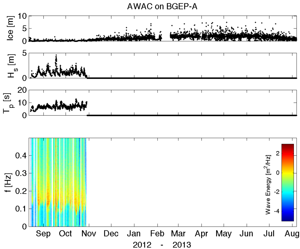
Figure 2. Ice thickness, wave height, wave period, and wave energy spectra from the AWAC on Beaufort Gyre mooring ‘A’.
