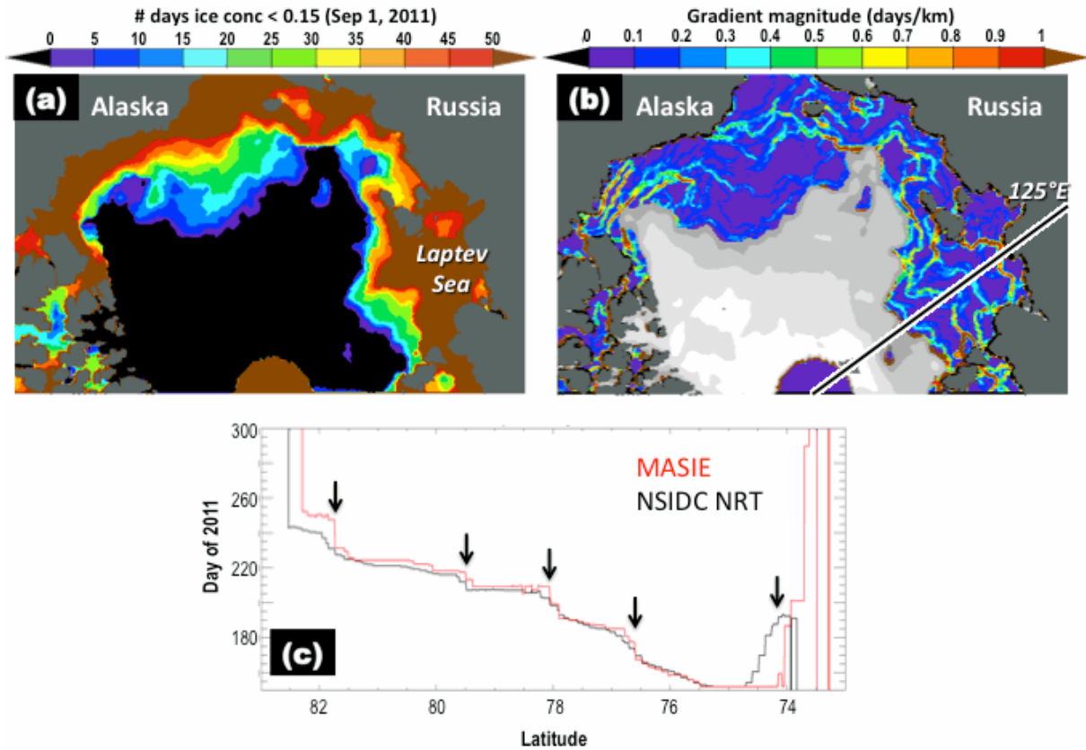
Figure 5. An example of sea ice retreat patterns for summer 2011. Panel (a): Number of days “ice free” (i.e., concentration < 0.15) using NSIDC near-real-time (NRT) passive microwave daily data. Panel (b): The magnitude of the two dimensional spatial gradient of the field in panel (a). Panel (c): Earliest 2011 day of open water (NRT = concentration < 0.15; MASIE = no ice) as a function of latitude along 125°E (see panel b) using MASIE and NSIDC NRT ice fields. Downward black arrows indicate ice edge “loitering” where gradients in open water days (panel b) are high.
