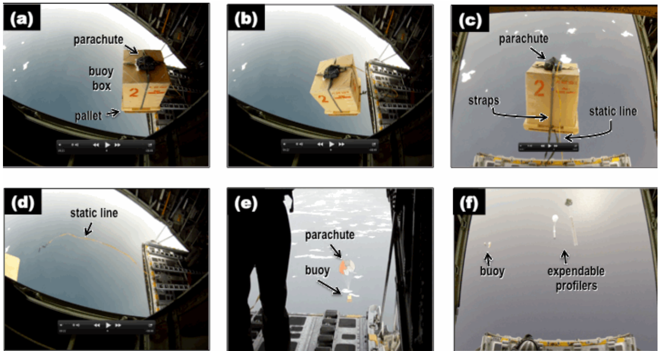
Figure 2. Deployment via C130 aircraft of the first SIZRS UpTempO buoy, August 13, 2013 by the Alaskan Coast Guard (CG) at 72N, 150W. (a) The buoy is packaged in a cardboard box strapped to a wooden pallet (below) and a parachute (above). CG personnel push the buoy out the aircraft's back door along rollers (a, b, c) when over the target drop location at an altitude of 200-500 feet. A static line releases the parachute (c, d, e). (f) Another pass is then performed for co-located deployment of expendable profilers (AxCTD, AxCP). Images from video shot by Dr. I. Rigor, PSC/APL/UW.
