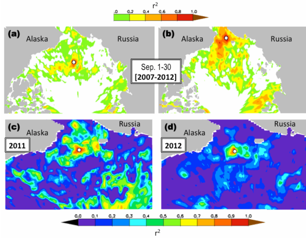
Figure 4. Upper panels: Correlation between the time series of Reynolds SST at a single location (white dot) over the month of September (averaged over 2007-2012) for (a) the Chukchi Borderland and (b) the Chukchi Sea, and all other locations. Lower panels: Same as upper panels, but for two individual years (c) 2011 and (d) 2012 in the northern Chukchi Sea.
