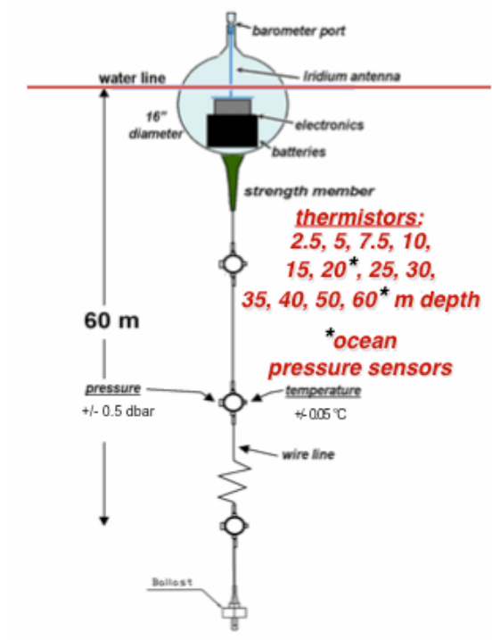
Figure 1. SIZRS air-deployable UpTempO buoy schematic.
