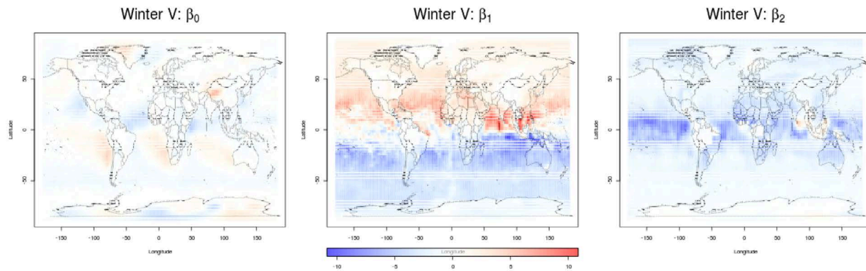
Fig. 3: Posterior means of model coefficients for V component of wind for winter data.
