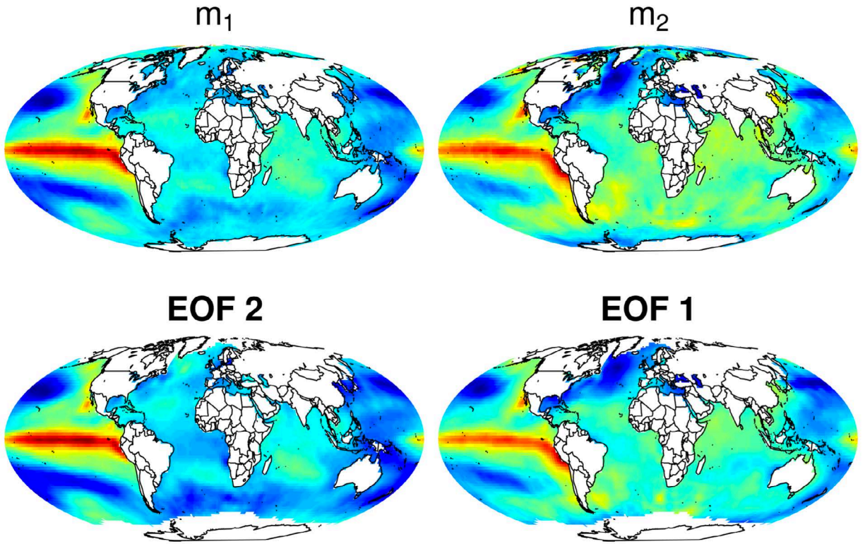
Fig. 5: Posterior mean fields and EOFs. Note that the ordering of the posterior mean fields, unlike EOFs, is arbitrary.
