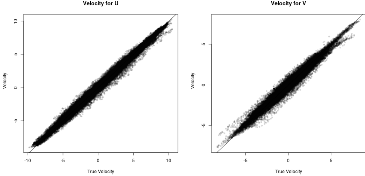
Fig. 4: Surface prediction vs. true wind velocity (m/s) for 10 years of data.
