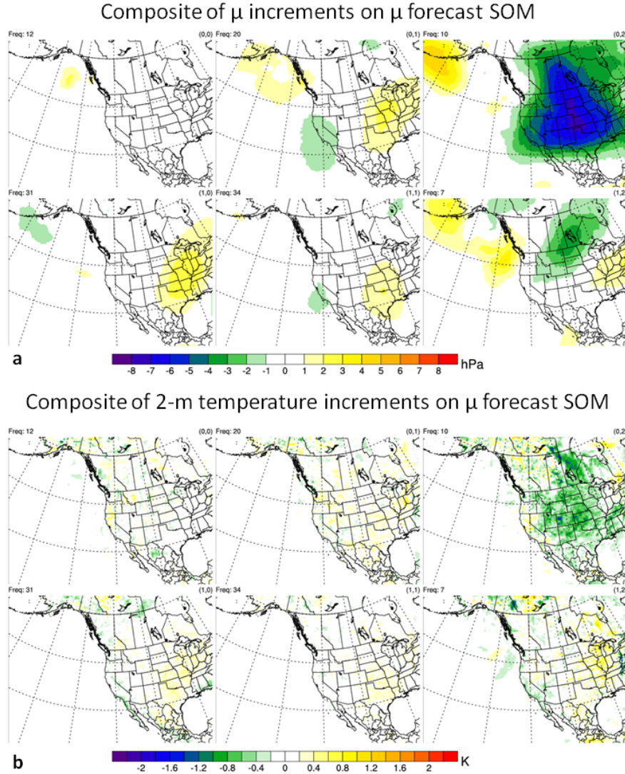
Fig. 1: Composites of (a) dry air mass ( \mu ) increments and (b) 2-m temperature increments for the dry air mass ( \mu ) forecast SOM. Frequency counts above each panel refer to the number of forecasts composited in each panel. The feature that stands out most in the \mu increment composite for the \mu forecast SOM (Fig. 1a) is the large negative increment over central North America in the composite for node (0,2). The \mu forecast SOM for that node exhibits ridging over central North America, and the composite increment is strongly negative. The combination suggests that the model systematically over-amplifies the ridge in the lee of the Rockies.
