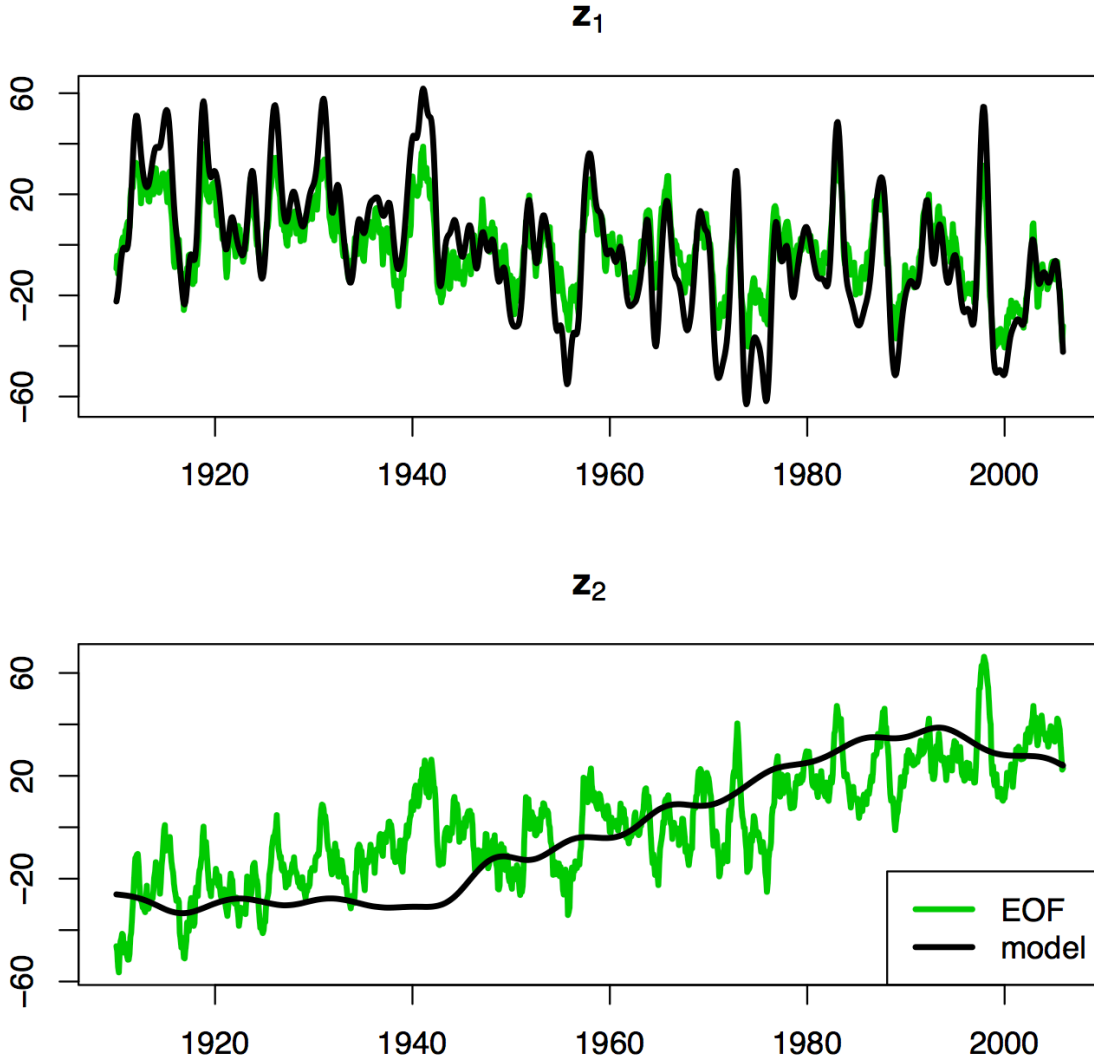
Fig. 6: Time series from hierarchical model (posterior means) and EOF analysis.
