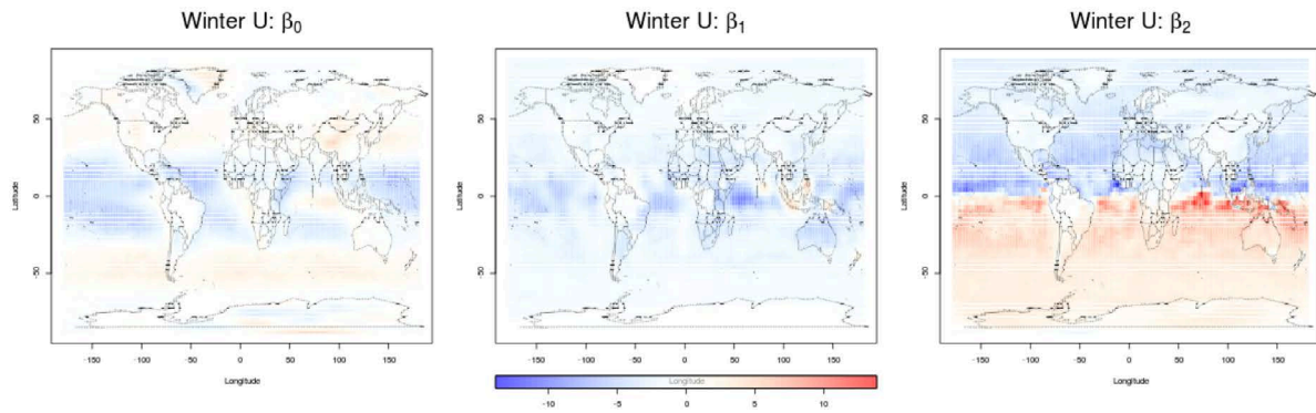
Fig. 2: Posterior means of model coefficients for U component of wind for winter data.
