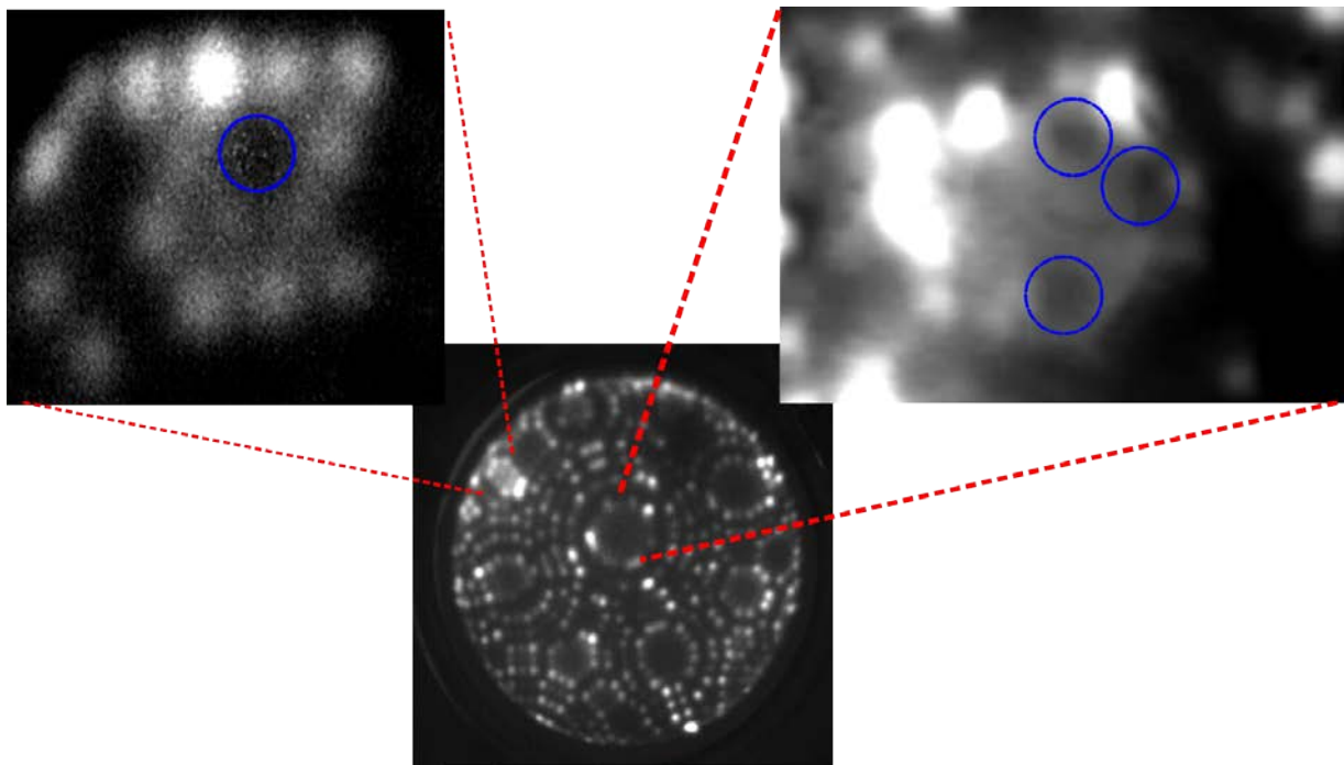
Fig.3. FIM pictures of tungsten surface. Top left: picture of (211) plane with surface vacancy (blue circle), created by \text{Ne}^+ ion sputtering. Top right: picture of (100) plane with surface vacancies (blue circles) created by \text{Ne}^+ sputtering. Bottom center: picture of a whole W(100) oriented tip.
