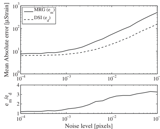
Figure 7. Mean absolute error of \varepsilon_{xx} over the interest domain and relative performance of direct strain imaging over meshless random grid ( \varepsilon_{yy} , \varepsilon_{xy} show similar behavior).
