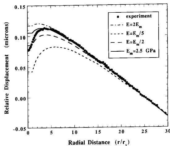
Fig. 5. Parametric studies of the effects of matrix modulus on the theoretical displacement profiles for no interphase.
