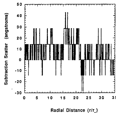
Fig. 10—Subtraction of two unheated scan lines yielding an average fluctuation of \pm 25\text{ }\text{\AA} about the horizontal line of zero displacement
