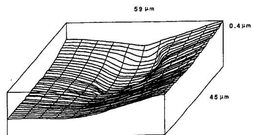
Fig. 7—Contour plot of initial unheated sample surface magnified 85\times
