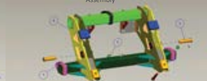
Bradley Protection Roller Interface Bracket Assembly
