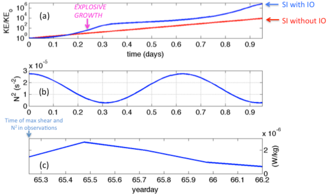
Fig. 3: (a) The KE of symmetric instability (SI) as predicted by a linear stability analysis (blue line) in flow field with similar characteristics to the observations, i.e. with negative potential vorticity, an inertial oscillation, and stable yet time variable stratification (shown in panel (b)). The KE of SI in a flow field without an inertial oscillation but with the same PV is also shown in the panel (red line). The interaction of SI with the inertial oscillation leads to periods of explosive growth that occur a little less than half an inertial period after the peak in stratification. Large eddy simulations configured with a flow similar to that used in the linear stability analysis illustrate that during these periods, SI develops secondary shear instabilities that enhance turbulence. (c) The observed dissipation as estimated from the Lagrangian float indeed shows that turbulent motions are intensified near yearday 65.5, a little less than half an inertial period after the peak in stratification.
