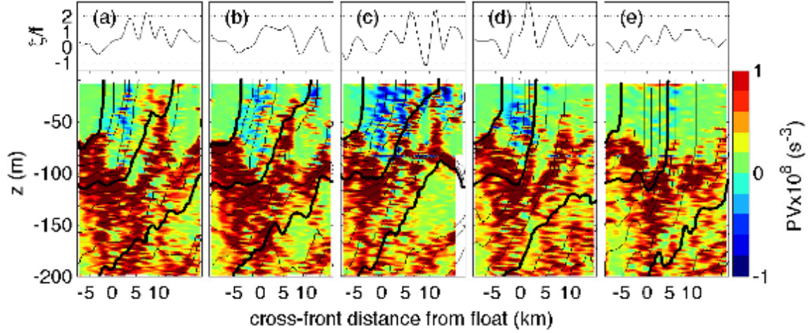
Fig. 2: A sequence of the vertical vorticity averaged over the top 60 m normalized by the Coriolis parameter (top panels) and cross-stream sections of density and potential vorticity (bottom panels). The sections were made on the R/V Atlantis around yearday 65.11 (a), 65.23 (b), 65.35 (c), 65.47 (d), and 65.61 (e). Density is contoured every 0.1 \text{ kg m}^{-3} and the thicker contours denote the 25.5, 26.0, and 26.5 \text{ kg m}^{-3} isopycnal surfaces. The presence of negative potential vorticity in a stably stratified boundary layer with positive vorticity indicates that the flow is symmetrically unstable. Note the steepening of isopycnals in the upper 60 m from yearday 65.35-65.61.
