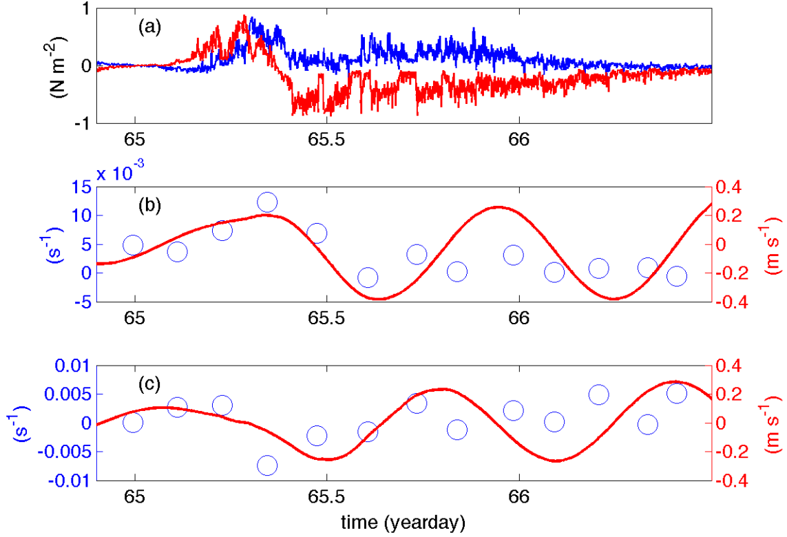
Fig. 1: Time series of the downstream (blue) and cross-stream (red) components of the wind stress (a), where downstream is defined to be in the direction of the float's drift. The down-stream and cross-stream components of the vertical shear (blue circles in (b) and (c), respectively) averaged across the top 60 m and horizontally over a cross-stream transect. The solution from a slab mixed layer model forced by the observed winds for the velocity in the downstream and cross-stream directions is indicated by the red lines in panels (b) and (c), respectively, and is scaled by the axis to the right in red. Before yearday 65.6 the observed vertical shears exhibit an inertial oscillation with similar phase and amplitude to the solution from the slab mixed layer model. After yearday 65.6, however, inertial oscillations are not evident in the observations, apparently having been dampened.
