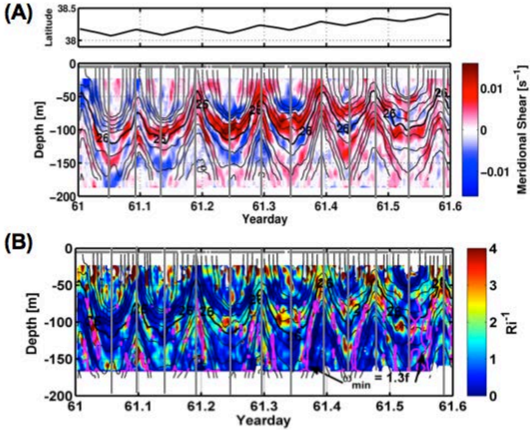
Fig. 4: Evidence of NIWs in the thermocline of the Gulf Stream and their potential for breaking. Depth-time series of density (contours), vertical shear of the meridional velocity (a) and the inverse Richardson number, Ri^{-1} , (b) on a Lagrangian drift from March 2-3 (yearday 61-62). The bowl like structure of the fields is a consequence of the ship track (plotted at the top of (a)) crossing the front multiple times. Bands of strong shear, running nearly parallel to isopycnals and that oscillate at a frequency 1.2f are observed in the thermocline. At certain phases of these NIWs Ri^{-1} approaches a value of 4, i.e. the threshold for breaking.
