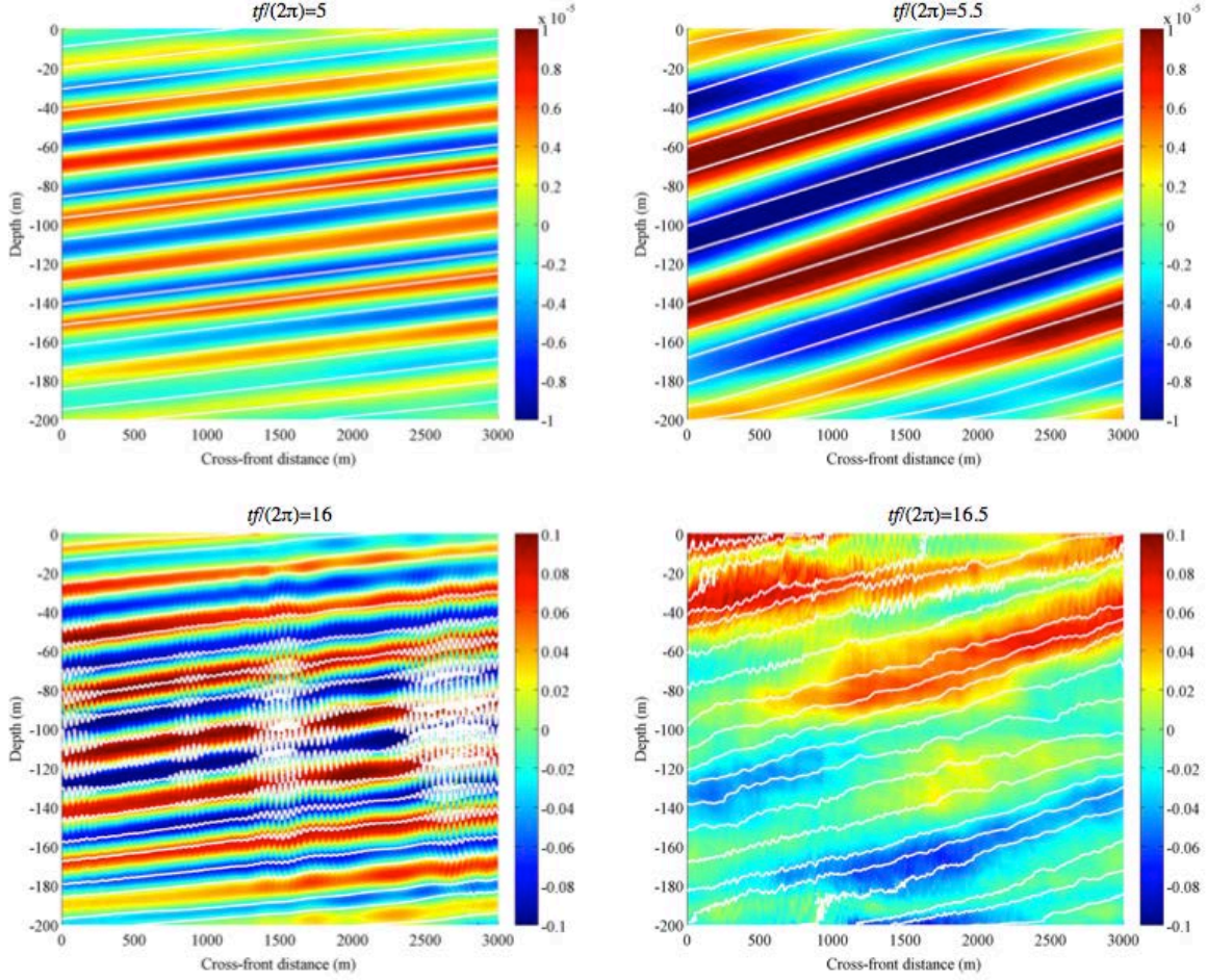
Fig. 5: Visualizations of the cross-front velocity (color shading) and isopycnals (white contours) from a numerical simulation illustrating the parametric subharmonic instability that can grow off of an inertial oscillation in a front. The upper row shows a time during the linear phase of the instability, with nearly along-isopycnal motion, and at times of maximum (left) and minimum (right) stratification. The bottom row again shows times corresponding to minimum and maximum stratification, but now at a later time immediately following the onset of a secondary shear instability.
