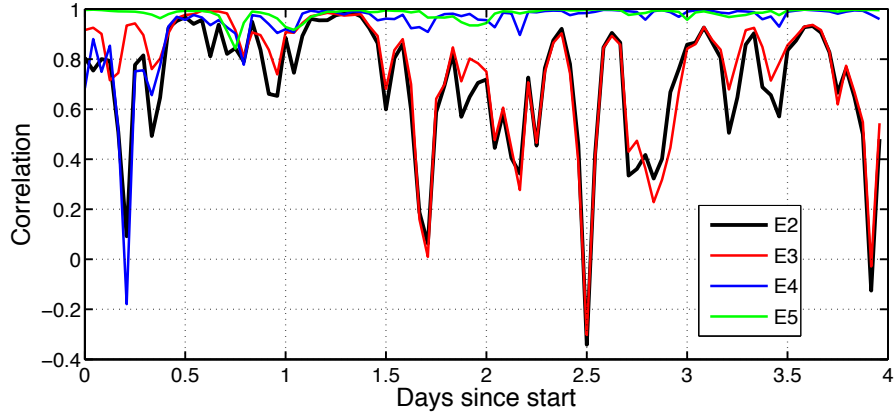
Figure 1: Correlation between various control vectors of the assimilation (initial conditions, boundary forcing, wind stress, and heat flux). For near coastal environments, we see that only when adjusting boundary conditions do solutions deviate from the prior prediction; hence, they are not initial value problems, as the initial field is swept away in less than 1.5 days.
