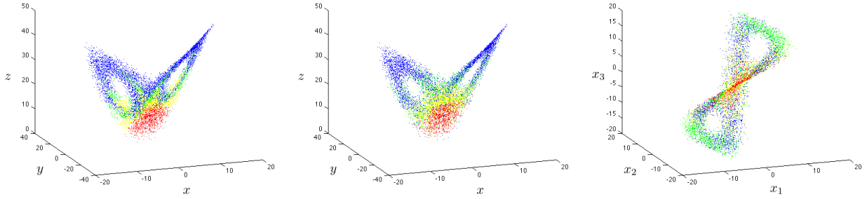
FIG. 1. (Color online) Growth rates of bred vectors in the Lorenz system using three different methods: (a) standard breeding in the phase space ( x ; y ; z ); (b) nearest-neighbor breeding in the phase space ( x ; y ; z ); and (c) nearest-neighbor breeding in the reconstructed phase space ( x_1 ; x_2 ; x_3 ). The colored points correspond to negative (blue), low (green), medium (yellow) and high (red) growth; see text for the value of the thresholds.
