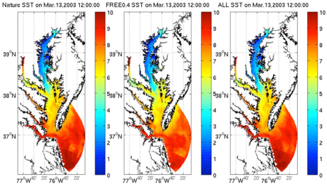
Figure 3. Comparison of Sea Surface Temperature for nature=truth (left), without data assimilation (middle), and with data assimilation (right)
