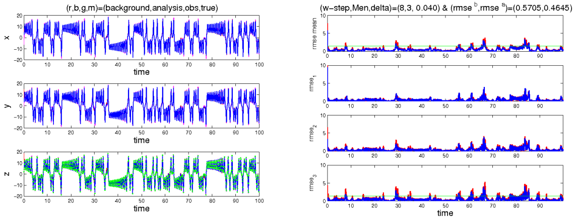
FIG.2. (Left) Forecast (red) and analysis (blue) using the most recent observed value (green) in the embedded space using the three-dimensional embedded space. (Right) corresponding root-mean square error.
