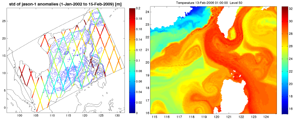
Figure 1. Left: South China Sea ROMS model domain and the pattern of Jason altimeter ground-tracks. Color indicates sea level variance. Right: Example of surface temperature in the environs of the Luzon Strait revealing mesoscale to submesoscale variability.
