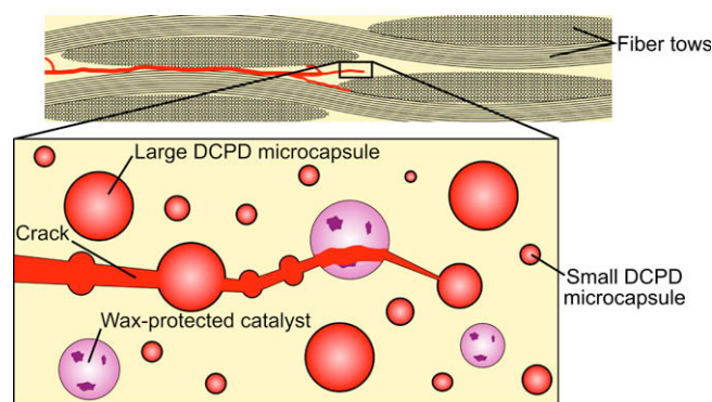
Fig. 1. Schematic of the self-healing system used in the matrix of a woven fiber-reinforced composite.
