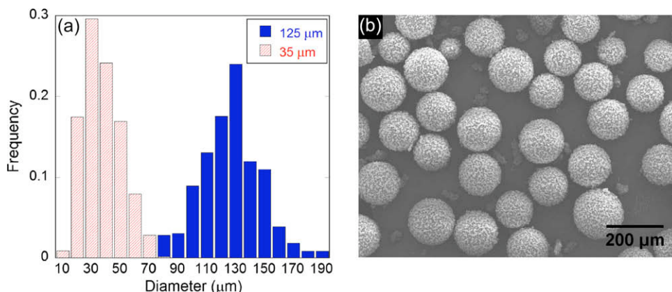
Fig. 2. (a) Histograms of microcapsule diameter for larger (125 μm) and smaller (35 μm) microcapsules used in this study. (b) SEM micrograph of larger DCPD microcapsules.
