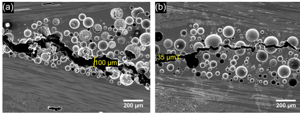
Fig. 10. Examples of the largest delamination separations seen in C-III panels impacted with (a) 45.1 J and (b) 17.8 J.
