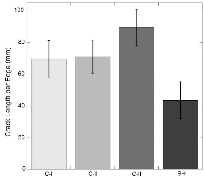
Fig. 7. Total crack length per imaged edge for plain (C-I), microcapsule-only (C-II), microcapsule and microsphere (C-III), and self-healing (SH) composite panels impacted with 45 J. Error bars are \pm 1 standard deviation.
