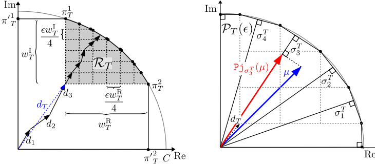
(b) Each in \{\sigma_i^T\} is a vector (starting at the origin) perpendicular to each boundary edge of \mathcal{P}_T(\epsilon) .
