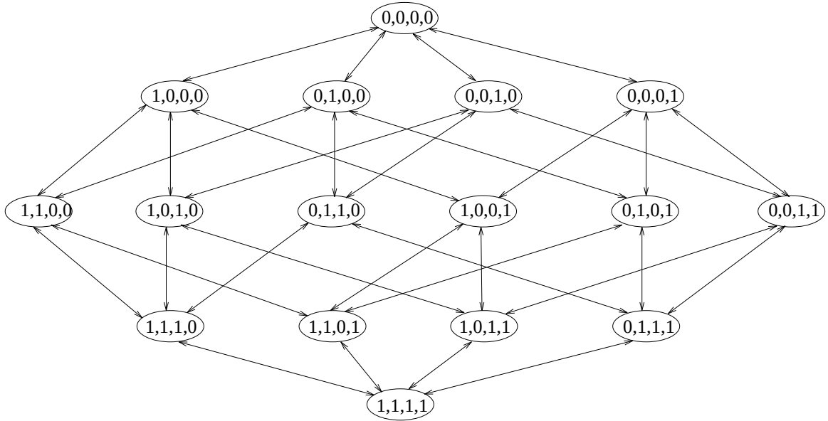
Figure 4.6: The state space search for feature subset selection. Each node is connected to nodes that have one feature deleted or added.
