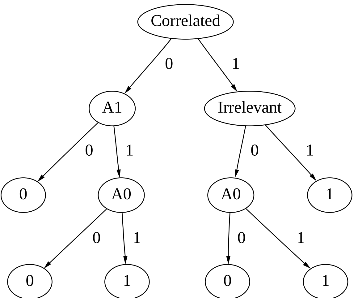
Figure D.15: The decision tree generated by C4.5 for corral. Accuracy: 81.25%. Note the split on the “irrelevant” feature and the root split on “correlated.”
