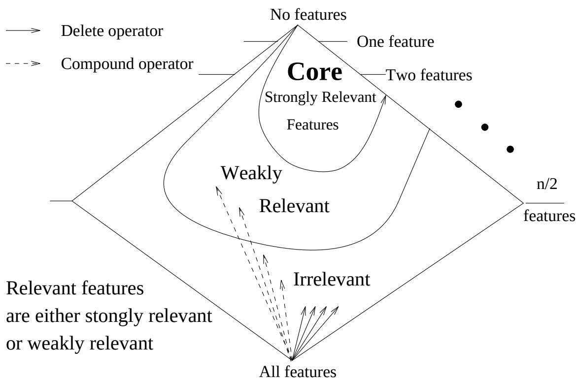
Figure 4.13: The state space. If a feature subset contains an irrelevant feature, it is in the irrelevant area; if it contains only strongly relevant features it is in the core region; otherwise, it is in the relevant region. The dotted arrows indicate compound operators.
