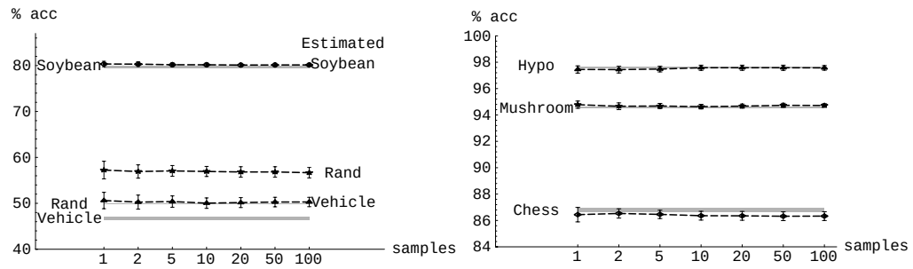
Figure 3.10: C4.5: The bias of bootstrap with varying samples. Estimates are good for mushroom, hypothyroid, and chess, but are extremely biased (optimistically) for vehicle and rand, and somewhat biased for soybean.
