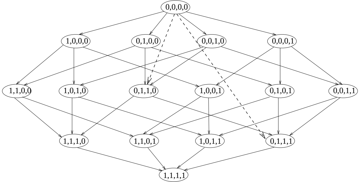
Figure 4.14: The state space search with dotted arrows indicating compound operators.
