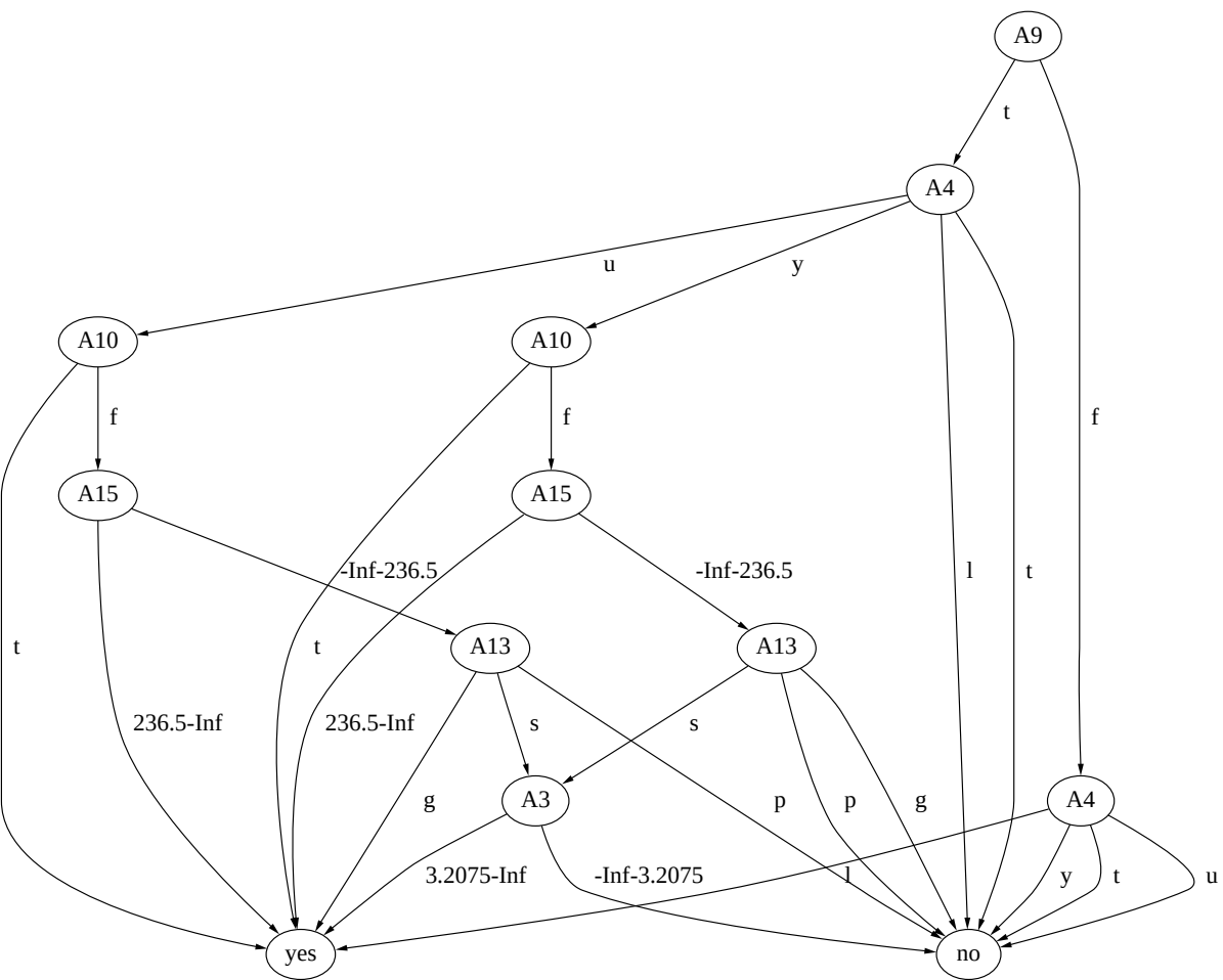
Figure D.6: The OODG generated by HOODG-Middle for Australian credit screening (crx). Accuracy: 84.04%.
