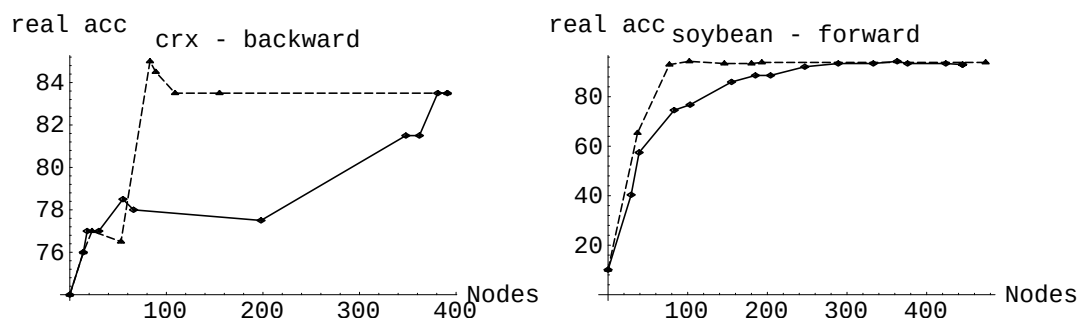
Figure 4.15: Comparison of compound (dotted line) and non-compound (solid line) searches. The accuracy ( y -axis) is that of the best node on an independent test set after a given number of node evaluations ( x -axis).
