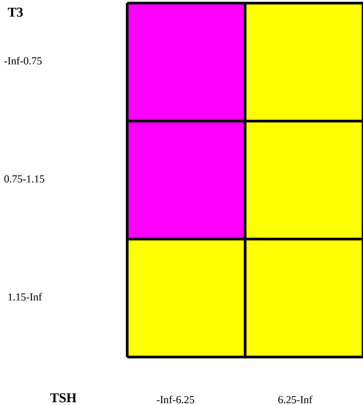
Figure B.7: The GLD for IDTM on dataset sick euthyroid. Accuracy: 97.35%
