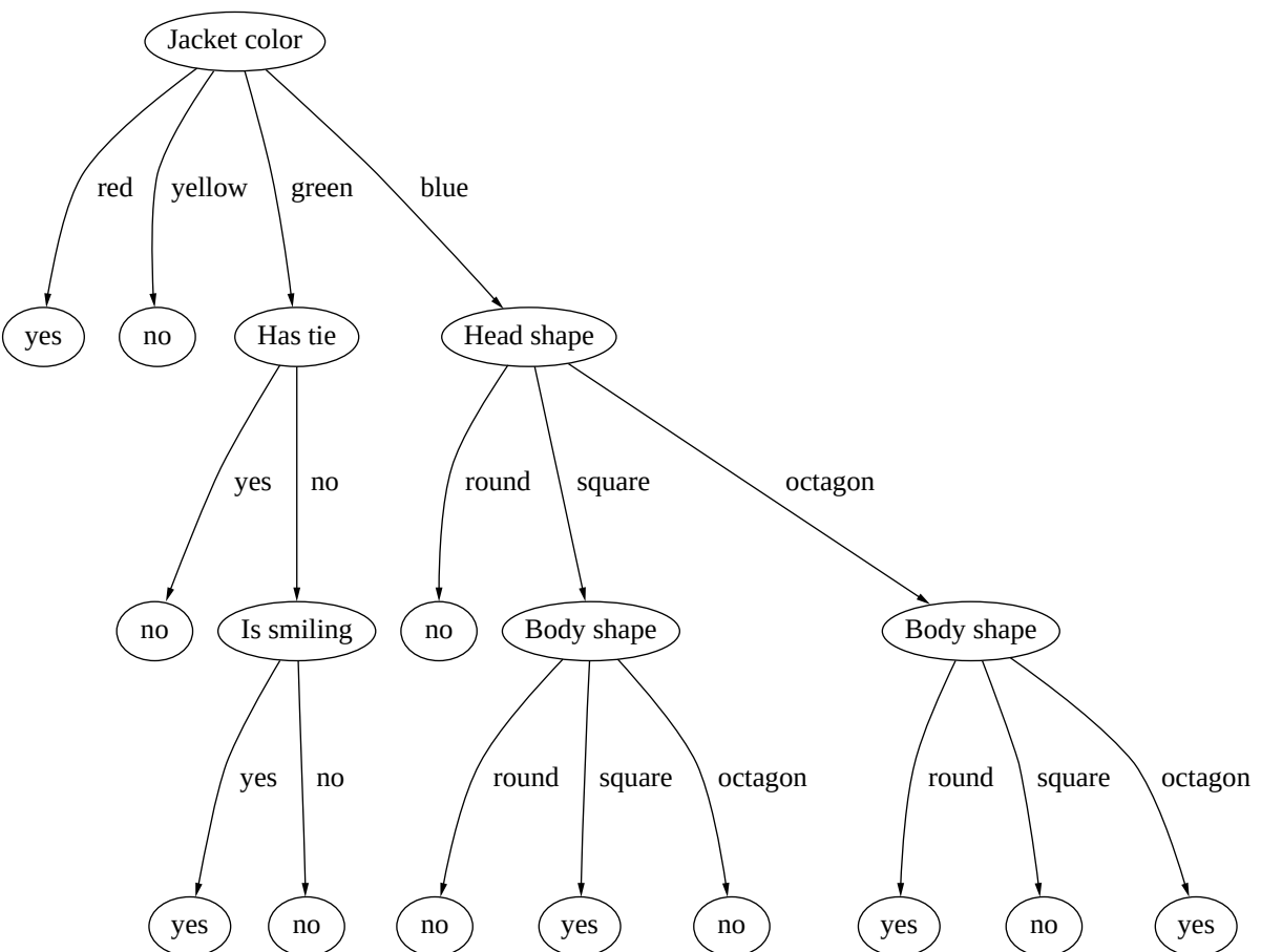
Figure D.19: The decision tree generated by C4.5 for Monk1. Accuracy: 75.69%.
