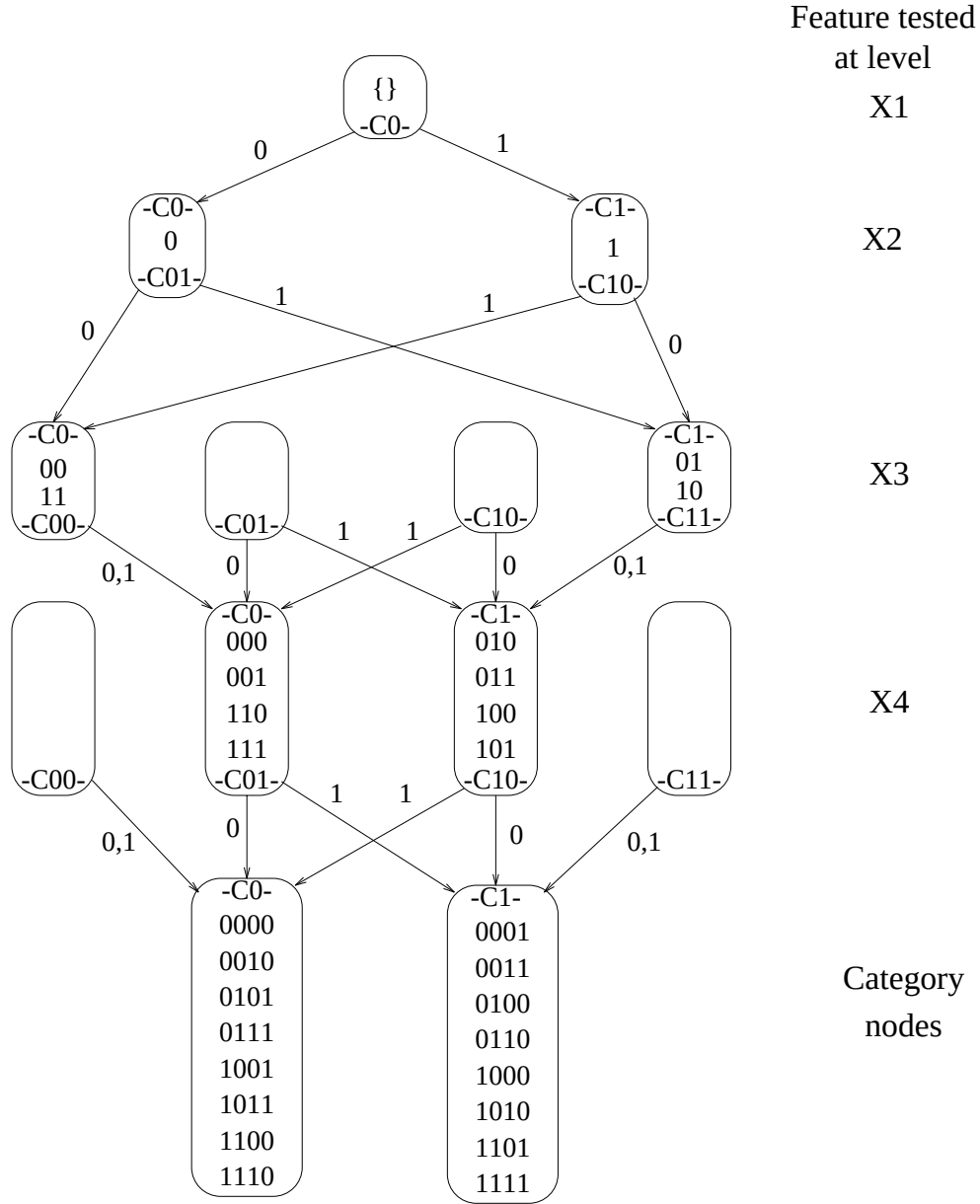
Figure 6.12: Example run of the bottom-up construction algorithm. The nodes correspond to the formed sets. The set name is represented at the bottom of each node ( e.g. , C_{10} branches to node C_1 at the next level on value zero and to node C_0 on value one), and the name used for the recursive call is at the top of each node. The target concept is f = X_1 \oplus X_2 \oplus X_4 .
