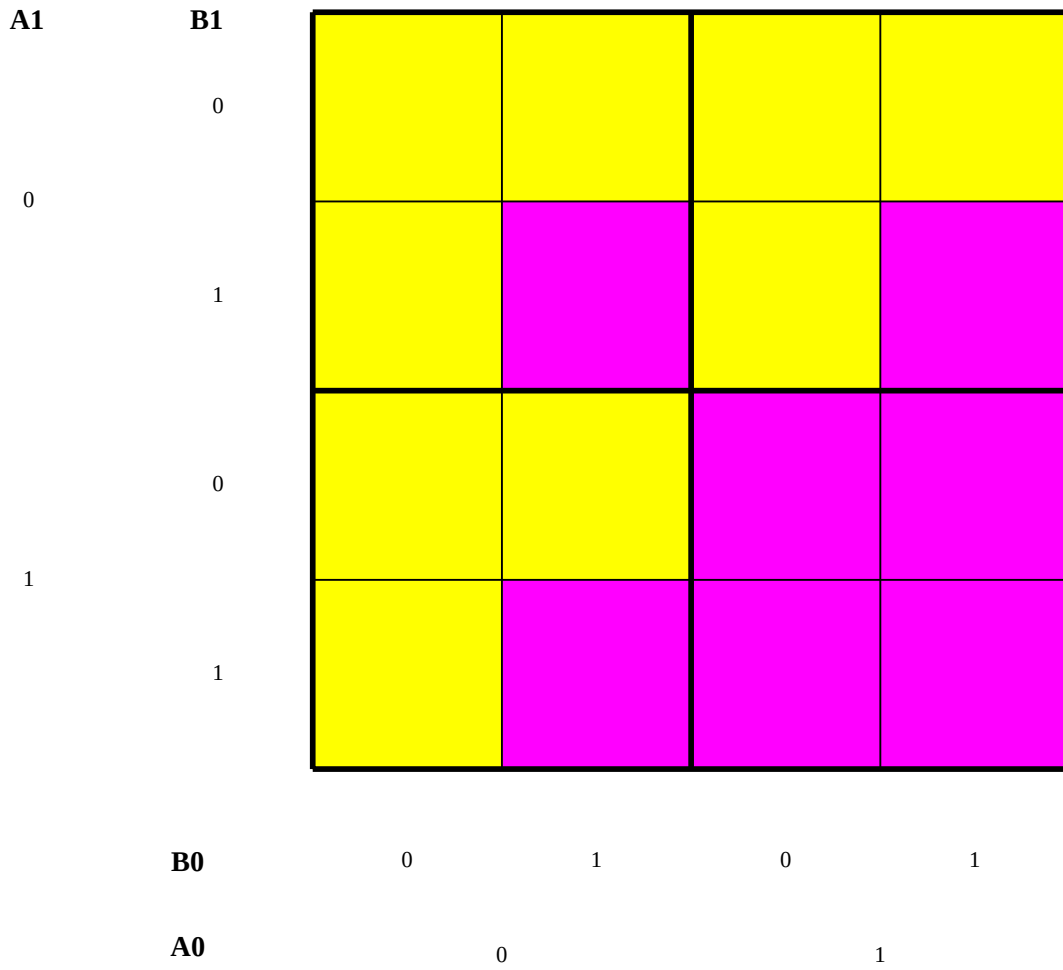
Figure B.8: The GLD for IDTM on dataset corral. Accuracy: 100.00%
