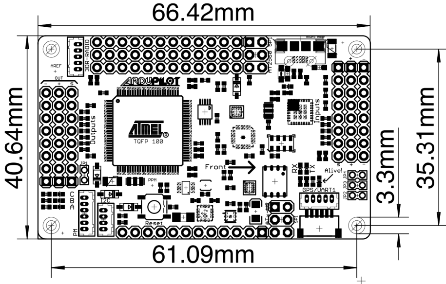
Figure 42: APM 2.5 Dimensions [16]
