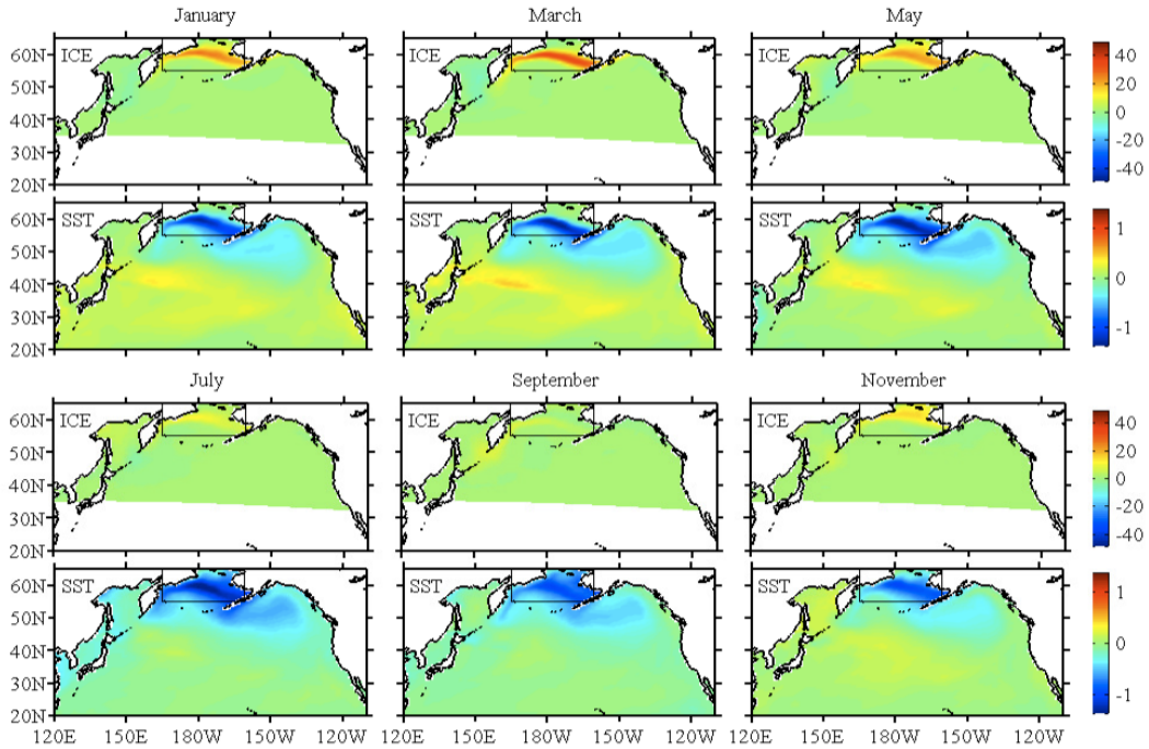
Figure 1: Sea Ice and SST patterns extracted using NLSA. The Bering Sea (boxed) exhibits a spring-fall sea ice reemergence. Positive spring sea ice anomalies imprint negative SST anomalies as they move northward during the melt season. The SST anomalies persist through the summer months, and when the ice returns in the growth season, the positive sea ice anomaly is reproduced.
