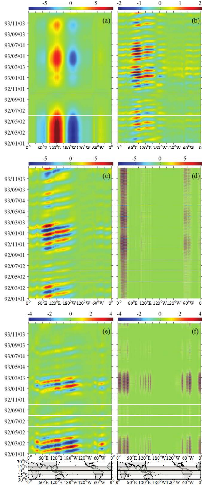
Figure 2: Multiscale spatiotemporal modes of the averaged temperature brightness field for 1992—1993 extracted using NLSA. (a) Symmetric interannual (ENSO) mode; (b) symmetric Maritime Continent mode; (c) symmetric MJO pair; (d) symmetric diurnal pair; (e) antisymmetric MJO pair; (f) antisymmetric diurnal pair.
