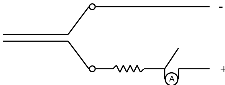
Figure 9. Standard “Y” Pattern Used in Electromigration and Dendritic Growth Testing
