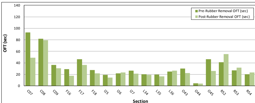
Figure 57. SH8000R Runway 22L pre- and post-OFT.
