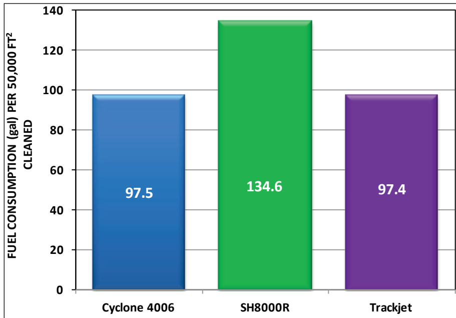
Figure 63. Fuel consumption.
