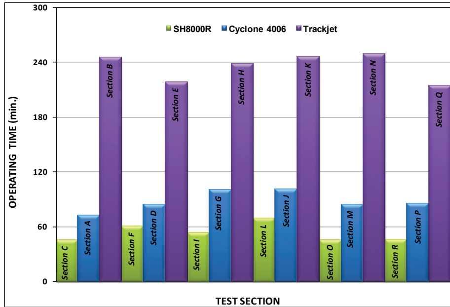
Figure 64. Elapsed test section cleaning times.
