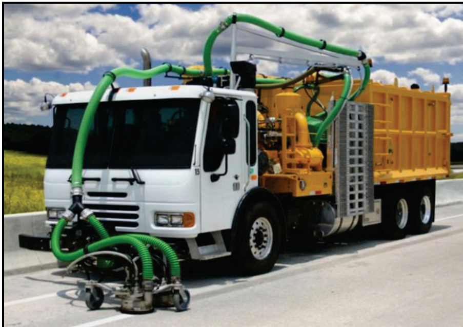
Figure 6. SH8000R rubber removal system.
