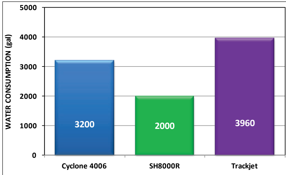
Figure 62. Water consumption.
