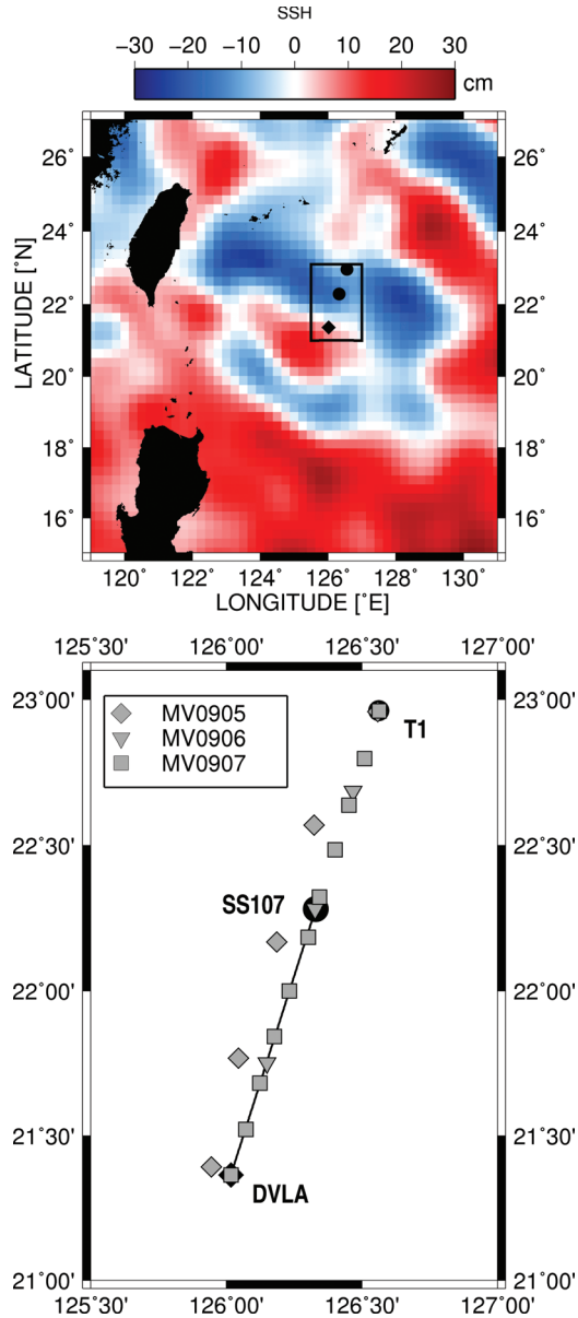
FIG. 1. Experimental plan for the PhilSea09 experiment. The top panel shows the region, including the islands of Taiwan and Luzon at 121^\circ E Longitude, 24^\circ and 17^\circ N Latitude, respectively. The color scale shows the sea-surface height for YD 119 of 2009 from the AVISO (Aviso and support from Cnes, 2012) database. The bottom panel shows the region bounded by the rectangle in the top panel. Sets MV0905, MV0906, and MV0907 denote CTD casts made on three consecutive 2009 cruises. The surveyed locations of the transmitter at station SS107 and the DVLA were 22.282\ 500^\circ N, 126.329\ 445^\circ E and 21.364\ 963^\circ N, 126.017\ 090^\circ E, respectively. The label “T1” refers to an acoustic transceiver mooring also deployed as part of PhilSea09, but is only shown here for context and will not be discussed in this work.
