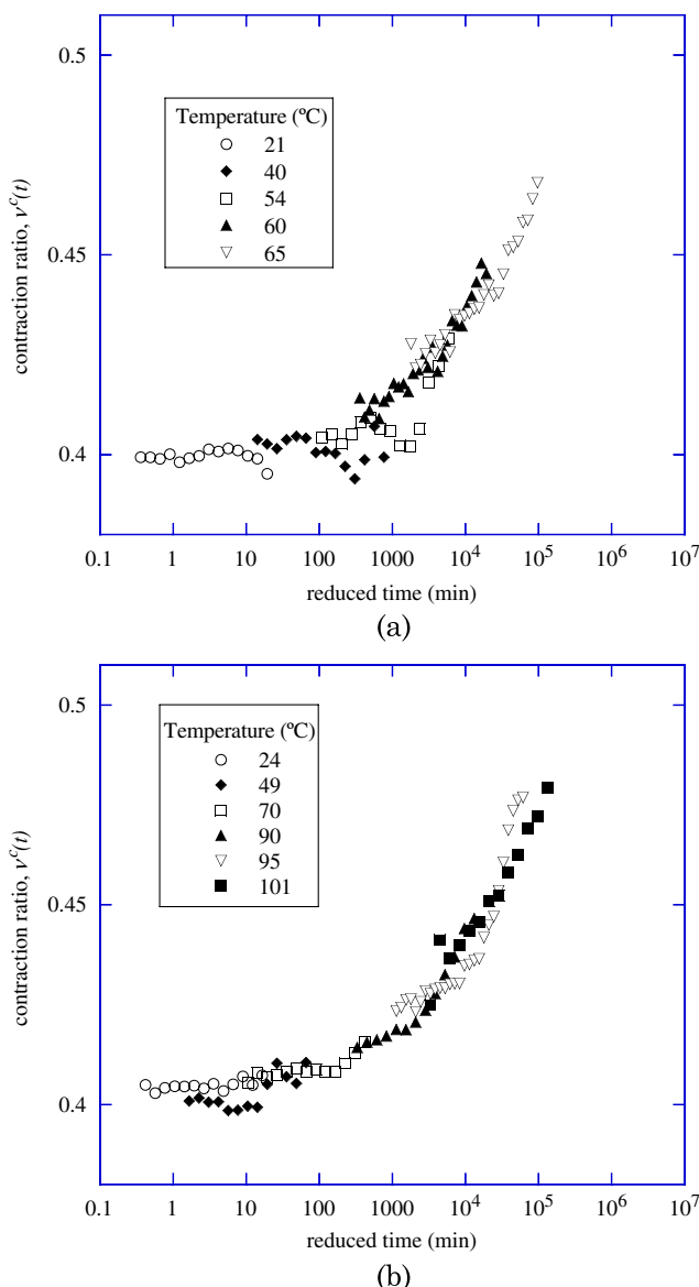
Fig. 13 Time-temperature superposition of lateral contraction ratio data for EPON 862/W, (a) \alpha = 0.79 ( T_{ref} = 21^\circ\text{C} ) and (b) \alpha = 0.90 ( T_{ref} = 24^\circ\text{C} )
