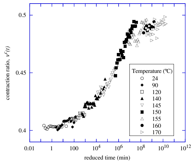
Fig. 10 Lateral contraction ratio in creep for EPON 862/W. Master curve was developed using same shift factors as creep compliance data ( T_{ref} = 24^\circ\text{C} )
