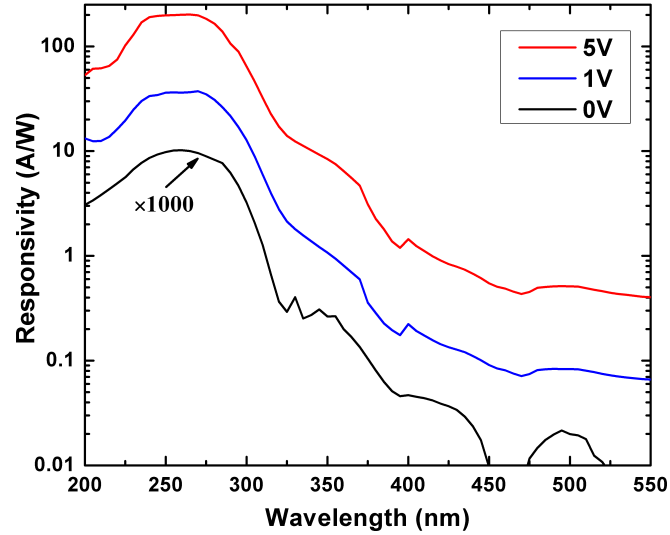
Fig. 13. Log scale plot of the responsivity of a MSM MgZnO photodetector with 5 \mu m pitch interdigitated electrodes at biases of 0, 1 and 5 V. The main optical cutoff is in the 280-300 nm range that corresponds to the fundamental optical absorption band in the MgZnO alloy. The small shoulder that appears near 310 - 375 nm is due to the photocurrent contribution from the thin ZnO buffer layer.
