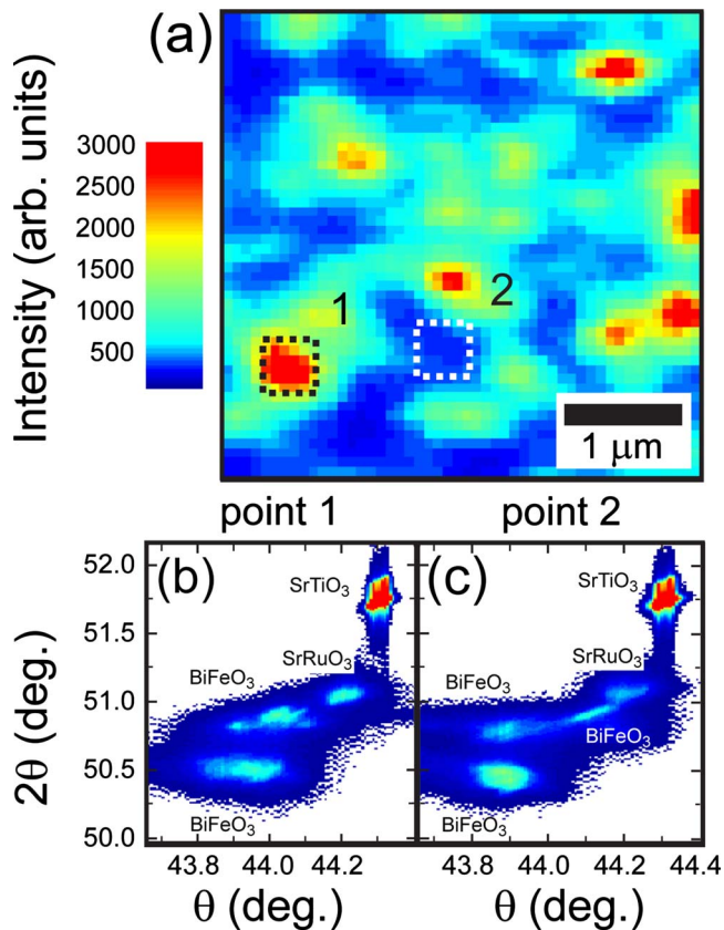
FIG. 4. (Color online) Microdiffraction image using the \text{BiFeO}_3 \{103\} reflections at 2\theta=50.73^\circ at the area marked 1. Reciprocal space maps taken at positions 1 (b) and 2 (c) on the surface. There are at least two \text{BiFeO}_3 \{103\} reflections, arising from the presence of multiple polarization domains within each mosaic block.
