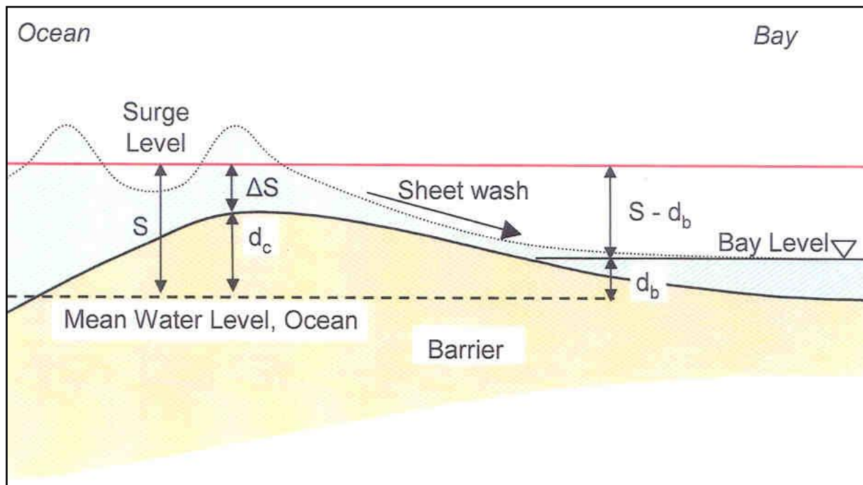
Figure 7. Definition sketch showing cross section of a barrier beach subject to overwash by overflow where barrier is fully inundated.
