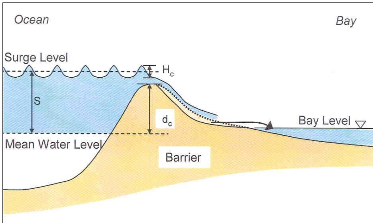
Figure 6. Definition sketch showing cross section of a barrier beach with a prominent dune subject to overwash by overflow.
