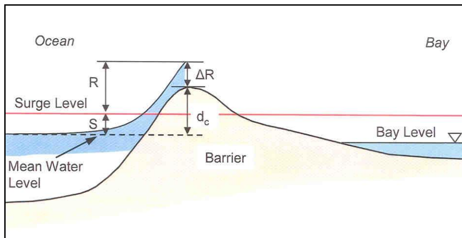
Figure 5. Definition sketch showing the cross section of a barrier beach subject to overwash by wave runup.
