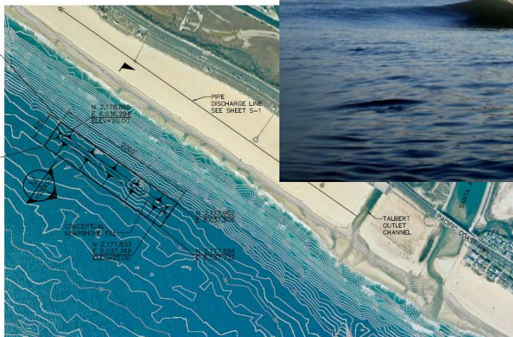
HUNTINGTON BEACH NEARSHORE CONCEPTUAL FILL PLAN VIEW 1"=500'
