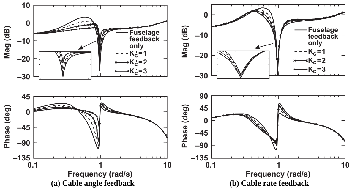
Figure 4-8. Aircraft response \phi/\delta_{lat} bode plot for combined fuselage and cable angle/rate feedback using constrained coupling numerators.
