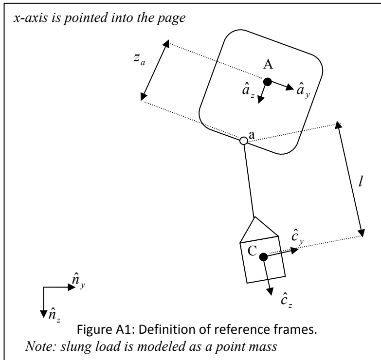
Figure A-1. Slung load geometry.
