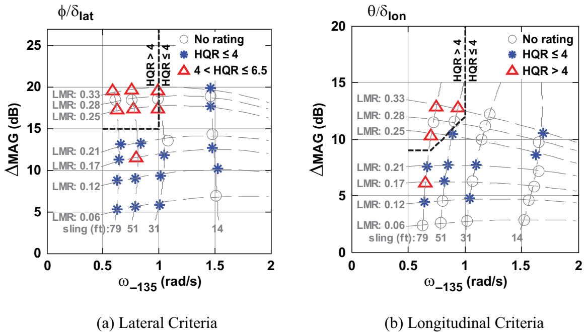
Figure 3-2. Slung load handling qualities criteria (Ref. 2), where HQR>4 represents poor handling.
