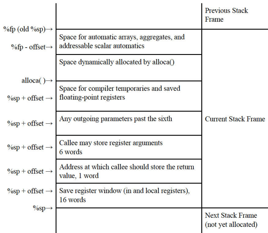
Figure 21: Memory stack of SPARC
