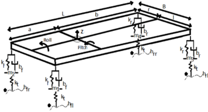
Figure 1 7DOF Vehicle Model Diagram
